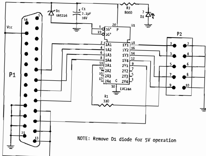
Figure 15-2: This reference schematic can be used to build a Blackcat cable.
