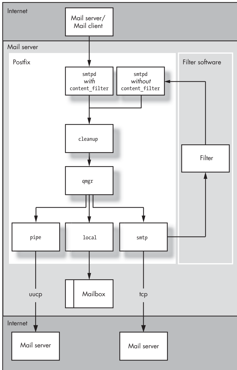
Figure 11-1: Delivery process using content_filter
