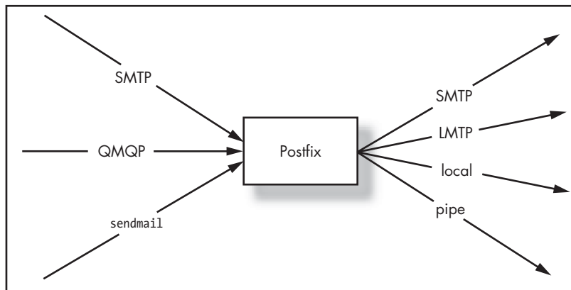
Figure 5-2: A Postfix "router" accepts and establishes all kinds of connections
