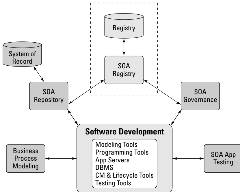
Figure 15-2: The repository, governance, and the registry.
