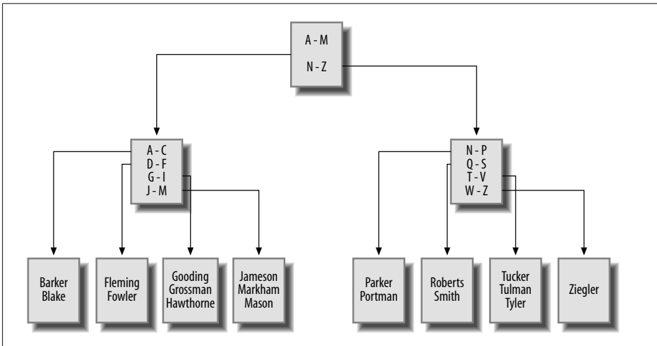
Figure 13-1. B-tree example
