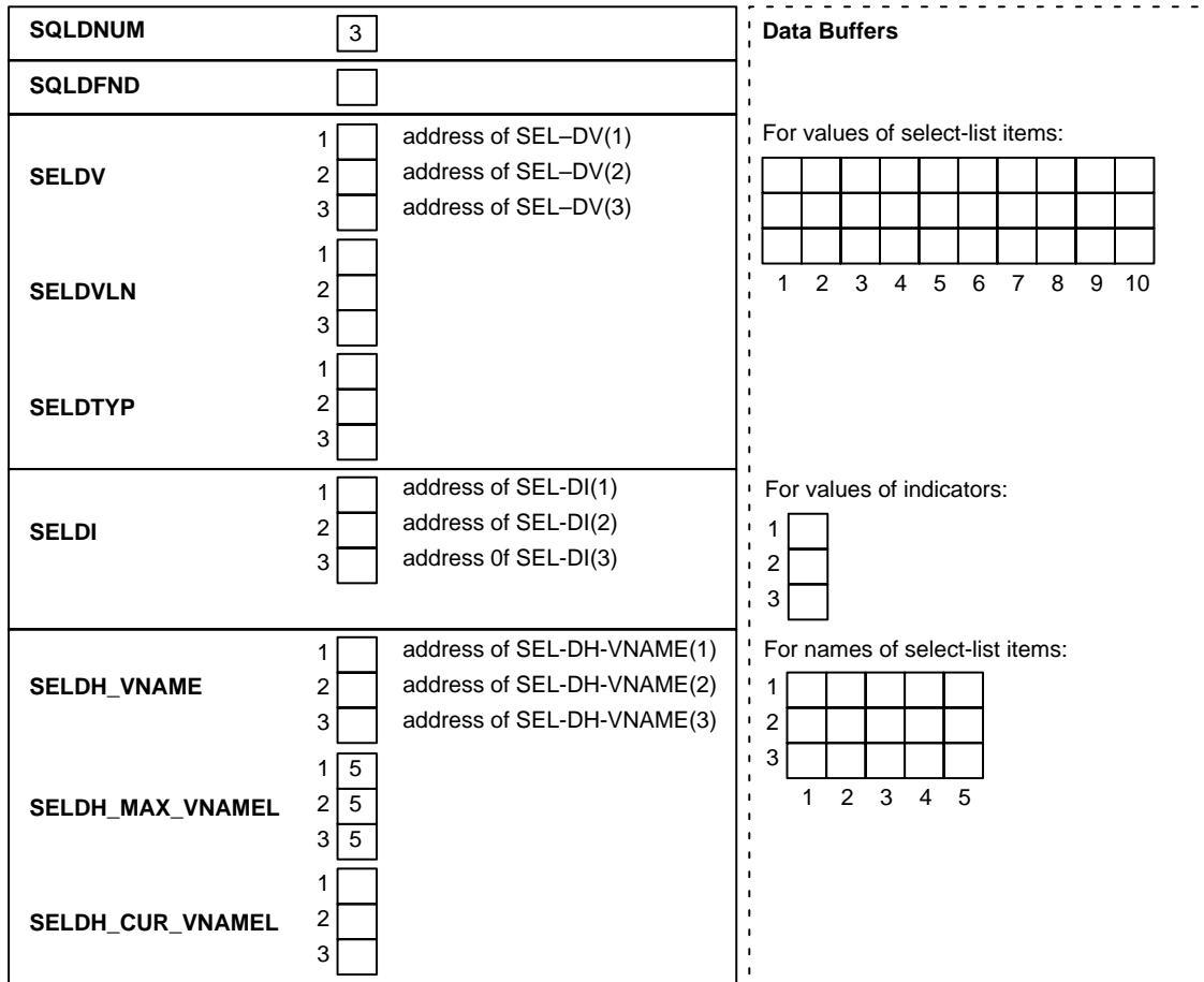
Figure 11-4 Initialized Bind Descriptor
