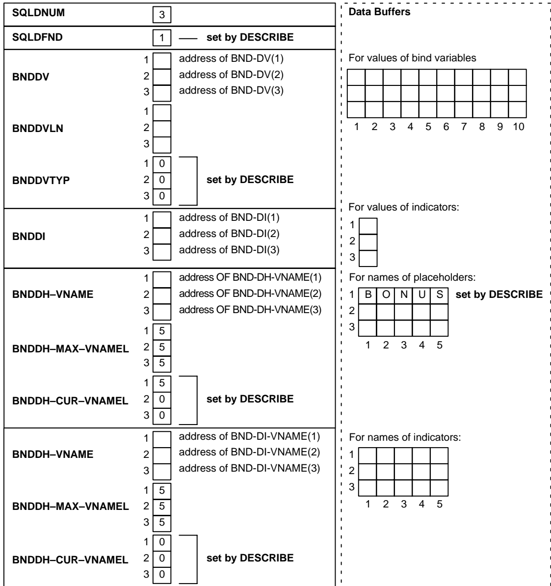
Figure 11-5 Bind Descriptor after the DESCRIBE
