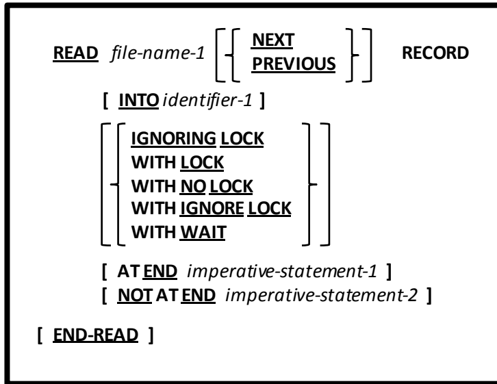
Figure 6-77 – READ (Sequential) Syntax
