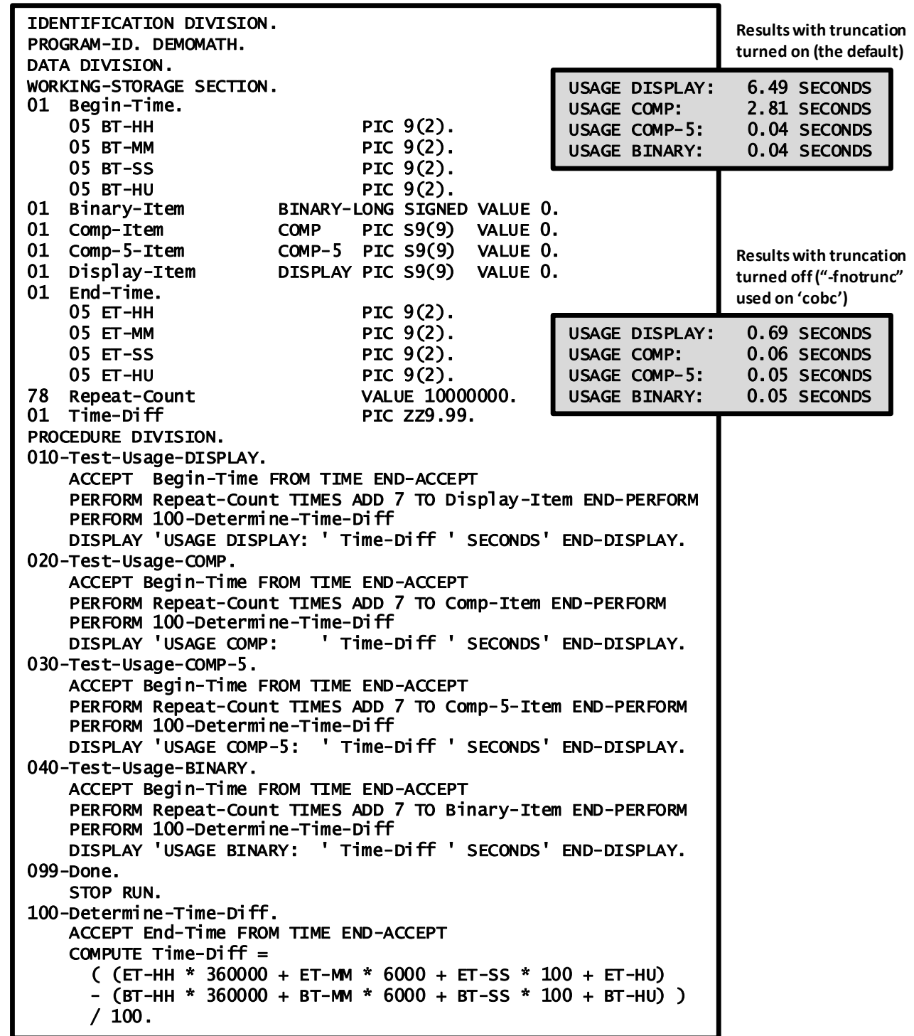
Figure 7-7 - A Non-Scientific Comparison of Numeric Data Item USAGE Performance
