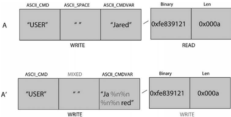
Figure 7.4 Session mutation.
