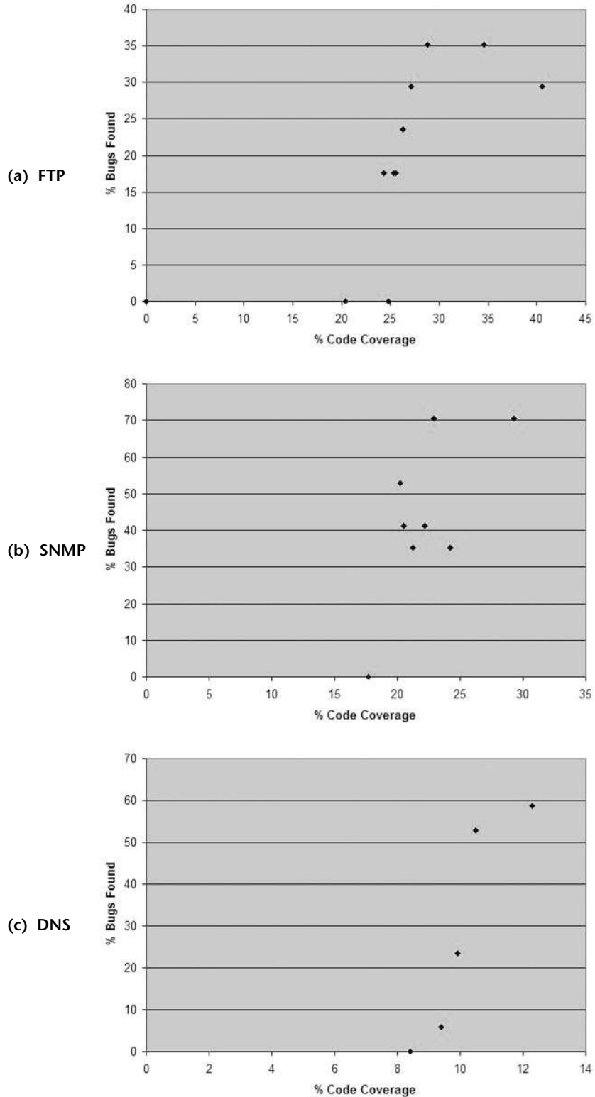
Figure 8.8 These three graphs plot code coverage versus bugs found for each of the fuzzers. Each point represents a fuzzer. The DNS graph especially shows the positive relationship.
