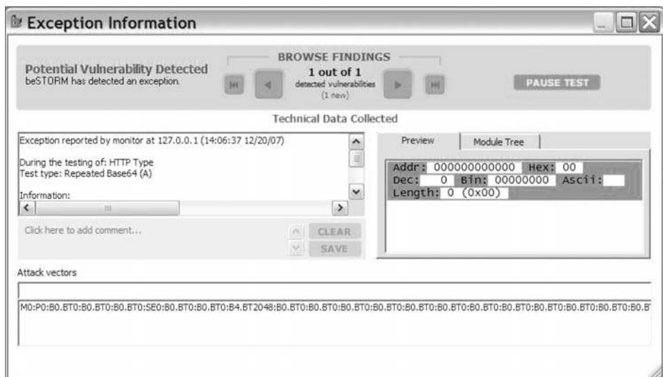
Figure 6.6 The beSTORM monitor reveals that it has detected a vulnerability.
