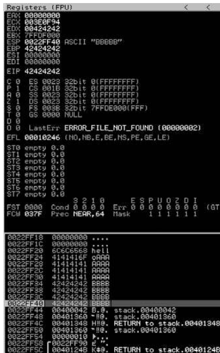
Figure 2.5 A register and stack trace from a debugger of above attack.
