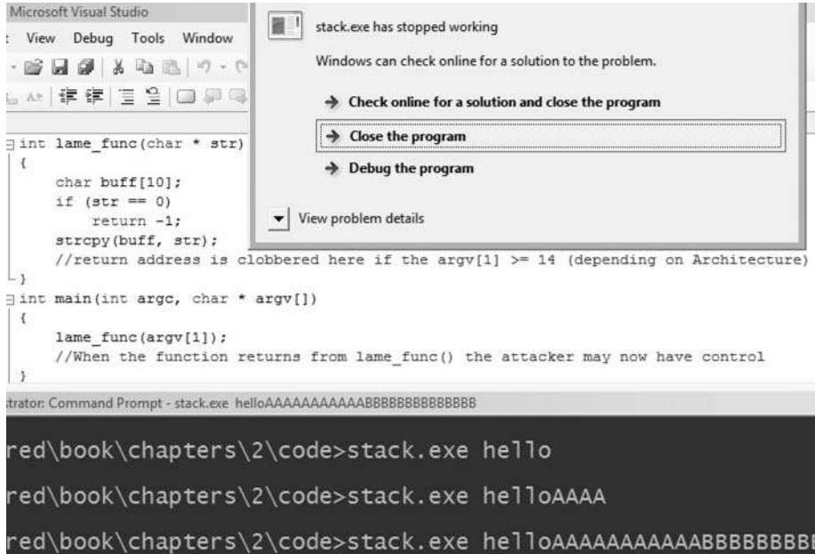
Figure 2.4 Demonstration of a stack overflow.
