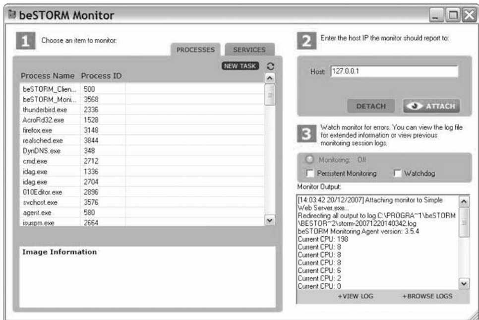
Figure 6.5 The proprietary beSTORM monitoring tool in action.
