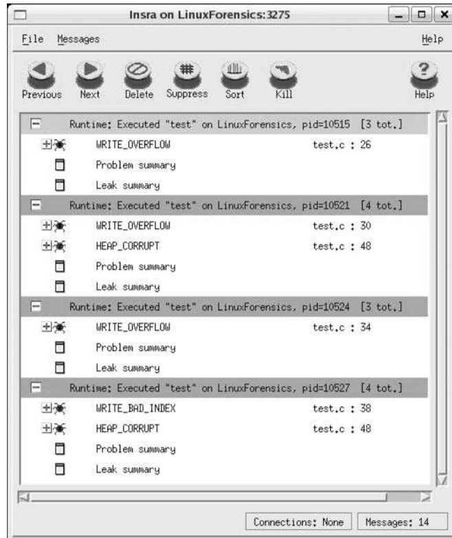
Figure 6.8 Insure++ reports on all issues it has helped detect.
