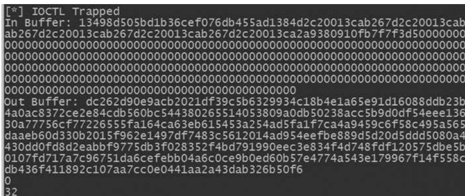
Figure 5.7 Output from ioctltrap.py.
