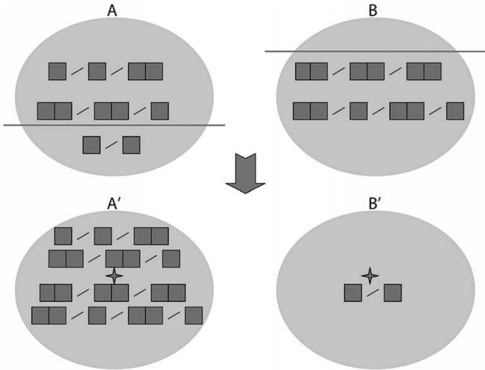
Figure 7.5 Pool crossover.
