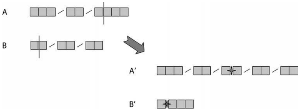
Figure 7.3 Session crossover.
