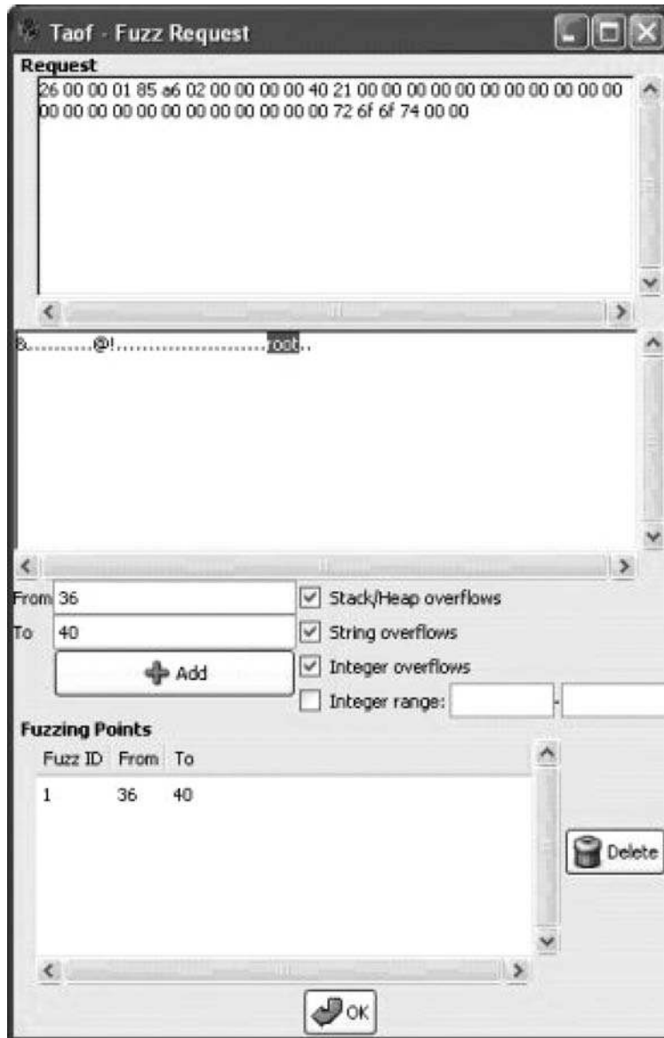
Figure 5.3 Adding fuzzing points.
