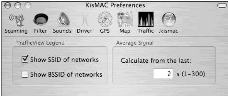
Figure 6.7 Traffic Preferences
