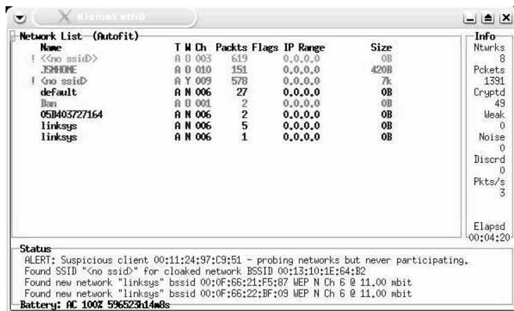
Figure 7.7 Kismet Interface
