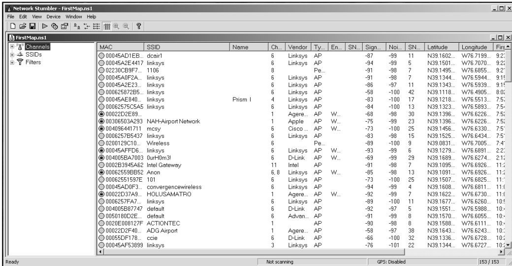
Figure 8.19 NetStumbler NS1
