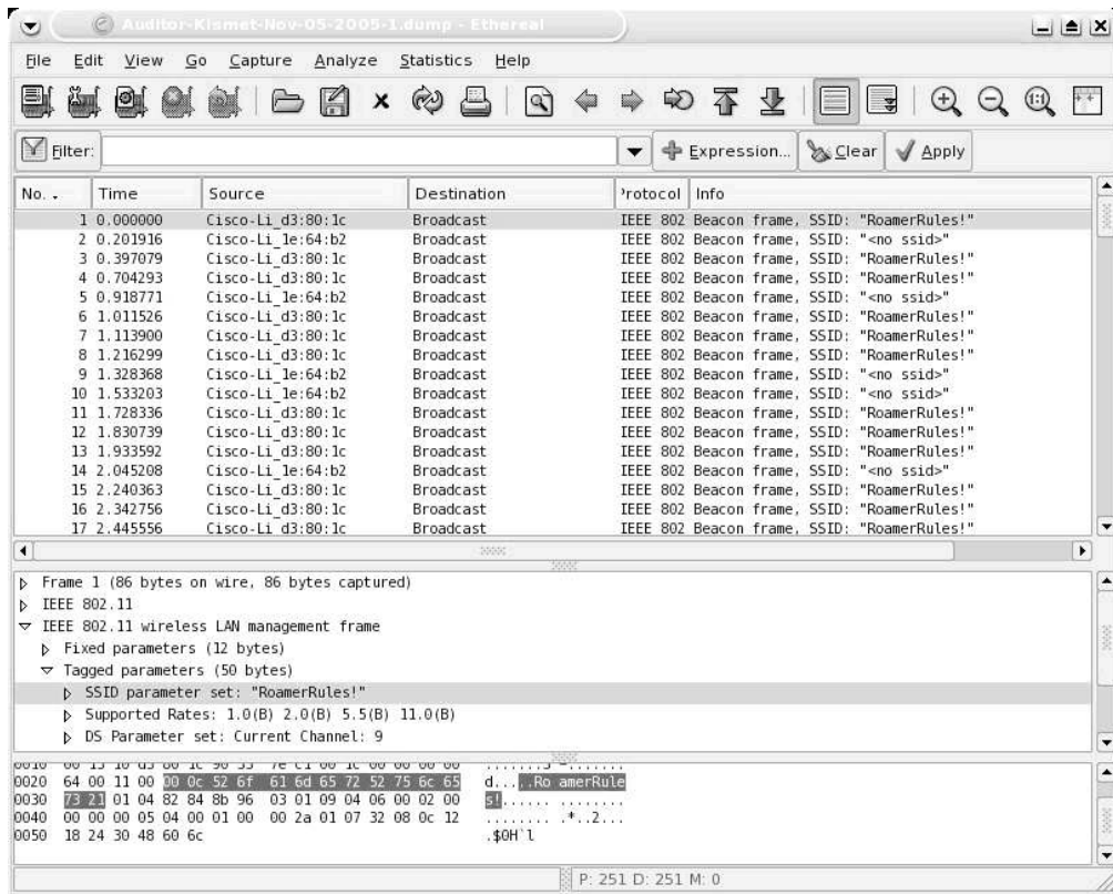
Figure 7.1 SSID Broadcast
