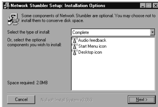
Figure 4.1 Installation Options
