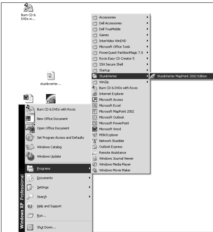
Figure 8.22 Starting StumbVerter
