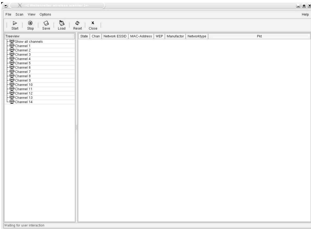
Figure 7.4 Wellenreiter Interface
