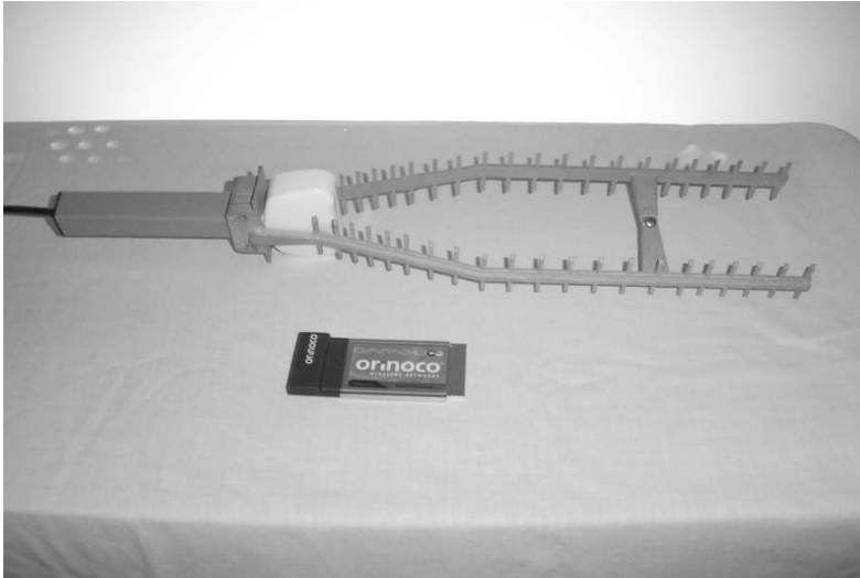
Figure 2.15 The “Vagi”
