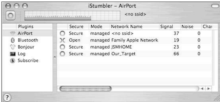
Figure 6.27 iStumbler
