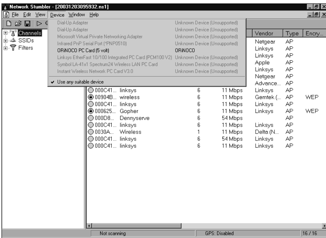
Figure 4.15 Device Menu
