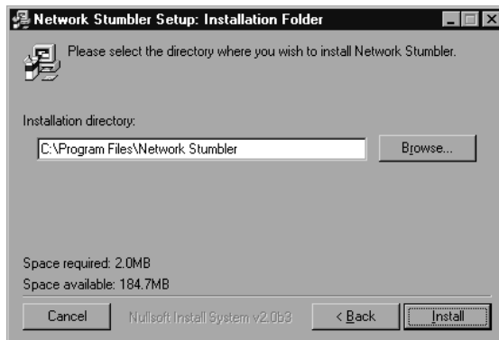
Figure 4.2 Installation Folder
