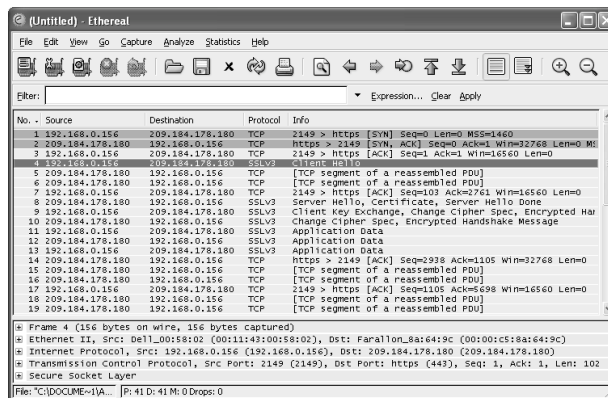
Figure 5.27 SSL Connection to Bank
