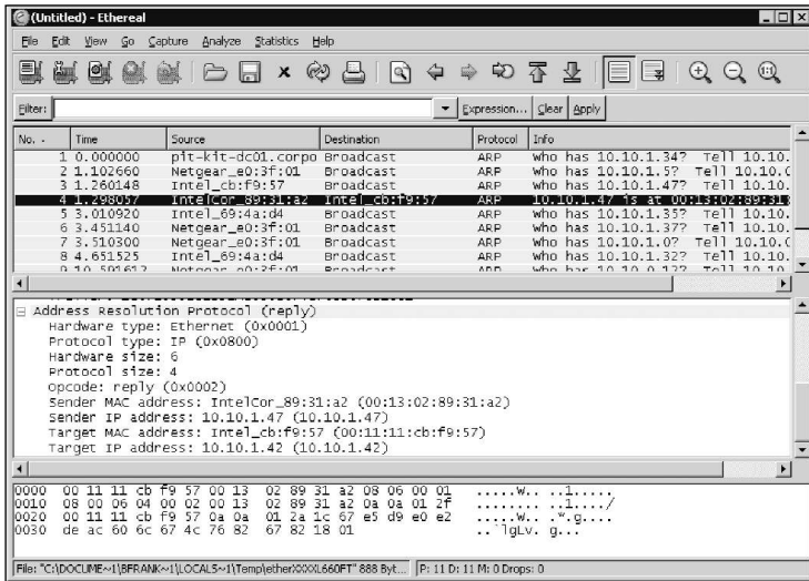
Figure 3.11 ARP Reply Packet
