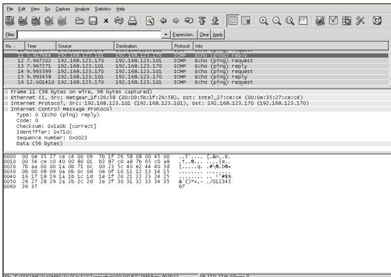
Figure 4.17 Linux Ping
