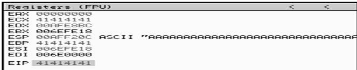
Figure 9.1 Crashing WS-FTP
