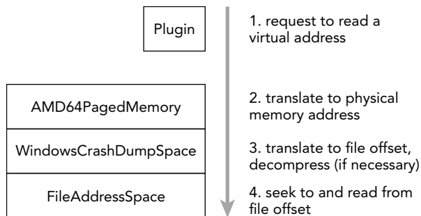
Figure 3-1: Volatility uses a stacked AS
