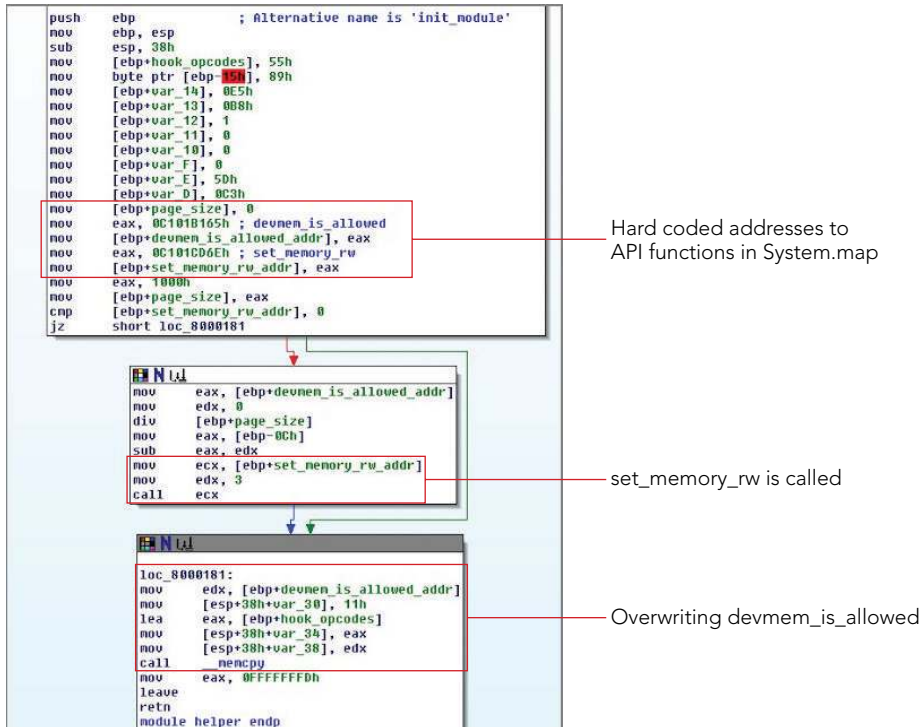
Figure 27-2: The module helper function of helper.ko
