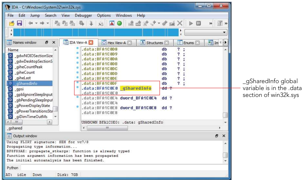
Figure 15-4: Analyzing win32k.sys in IDA Pro for clues on how to find the shared information structure
