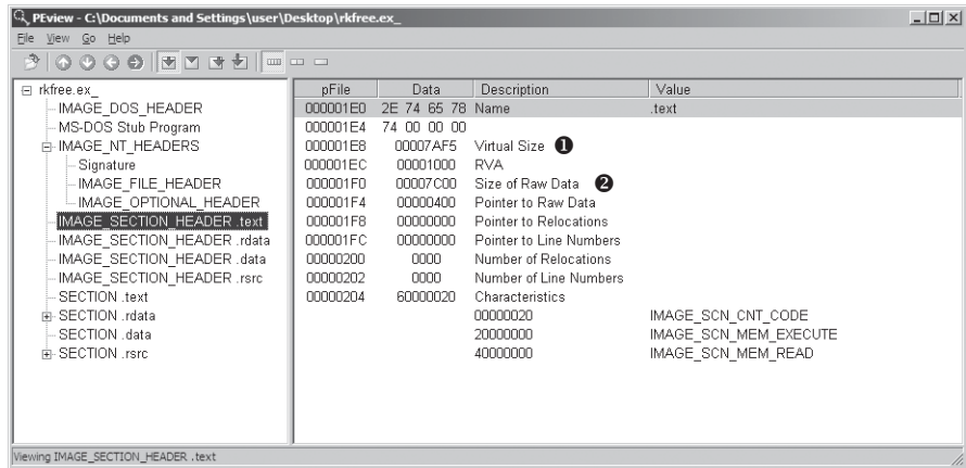
Figure 1-8: Viewing the IMAGE_SECTION_HEADER .text section in the PEView program
