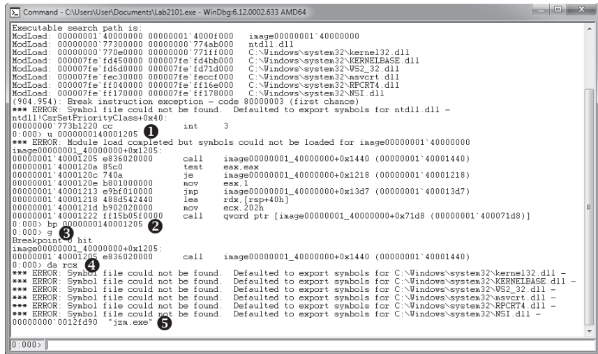
Figure 21-1L: Using WinDbg to see the string that is being compared in Lab 21-1
