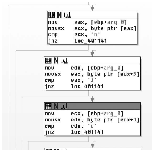
Figure 14-41: Obfuscated string comparison
