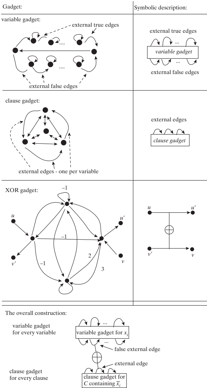
Figure 17.3. The gadgets used in the proof of Valiant's Theorem (Theorem 17.11).
