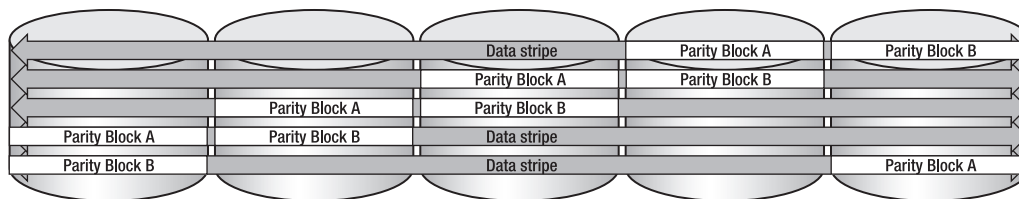
Figure 3–11. RAID 6
