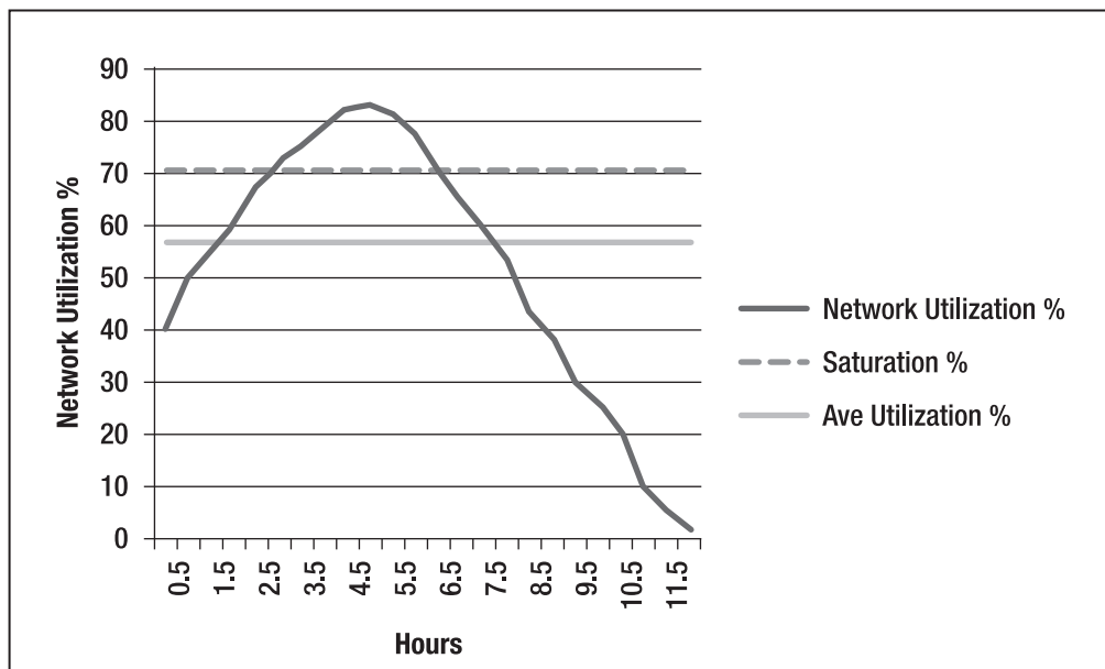
Figure 6–9. Network overutilization
