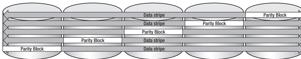
Figure 3–10. RAID 5
