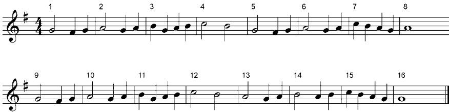
A sixteen-measure melody, consisting of four four-measure phrases.
