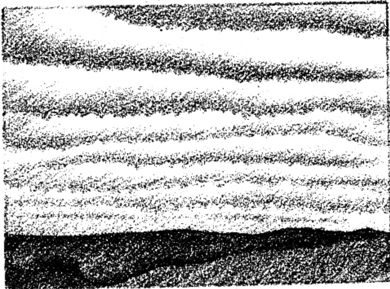
Stratocumulus
