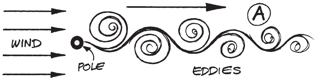
FIGURE 41 A Plan view of eddies formed as wind passes the pole. Each eddy is a cylinder roughly at right angles to the paper. B Wave shape of flag between left and right eddies. C Repeating animation cycle. The wave crest marked X follows itself along the flag ad infinitum.
