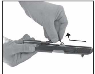
Fig. 10> Taking out the recoil mechanism (recoil spring with guide)
