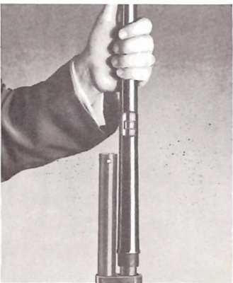
2 Align grooves on barrel shank with non-grooved areas in receiver.
