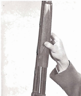
4 Replace forearm on magazine tube and seat against receiver. Take-down screw will enter hole in barrel lug.
