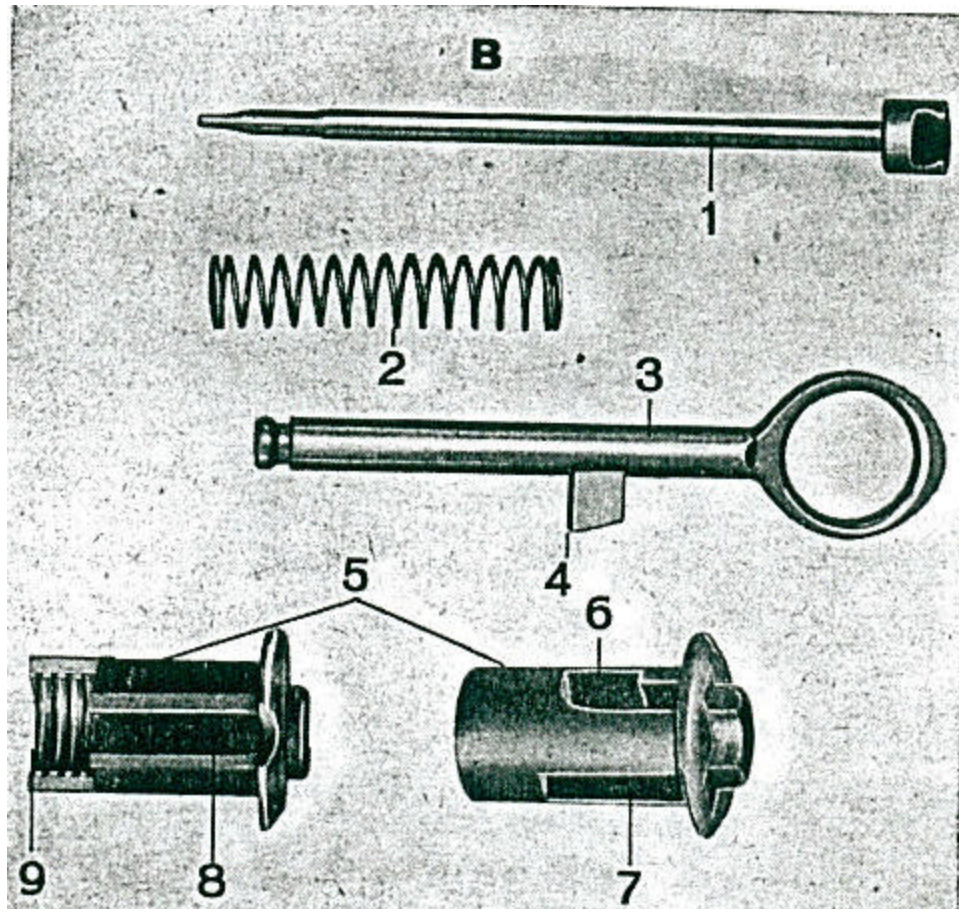
Fig. 12 Firing Mechanism
