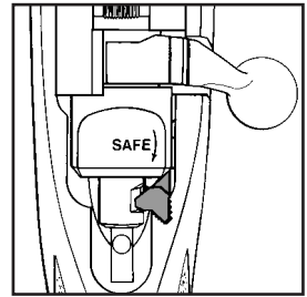
Figure 5. Safety selector in “SAFE” (full rearward) position. The safety selector is fully nested in the groove in the cocking piece. When the safety selector is in this position, the bolt handle cannot be raised. The curved arrow on the bolt sleeve indicates the direction and motion of the safety selector to bring it to the “SAFE” position. Keep the safety selector in this position except when actually loading, unloading, or firing.
