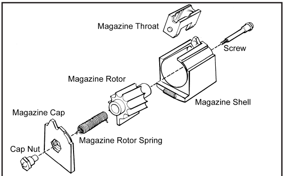
Exploded view of the 22 Charger Pistol magazine components. This illustration is included to show the relationship and names of the magazine components. As noted in the text above, the magazine should not be disassembled.
