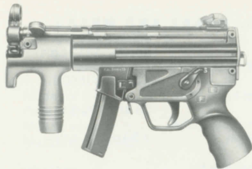
Fig. 54 MP5K Submachine gun
