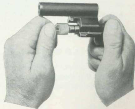
Fig. 36 Stripping the bolt assembly
