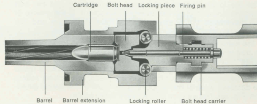
Fig. 29 Bolt in locked position
