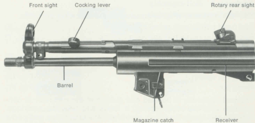
Fig. 4 Receiver with barrel, cocking mechanism and sights
