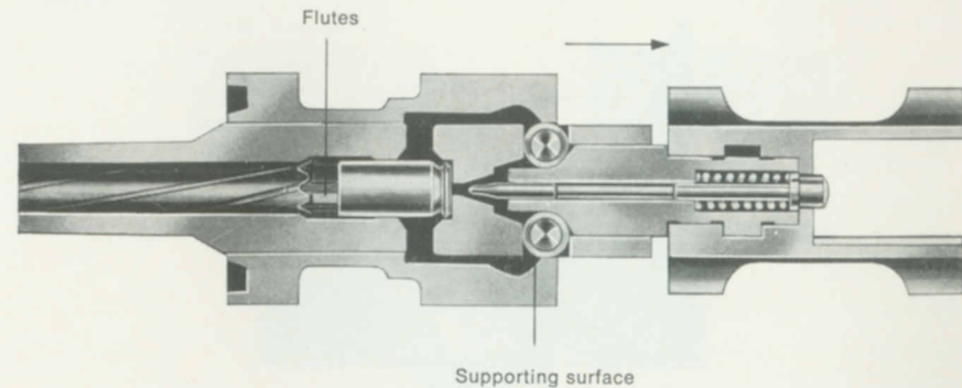
Fig. 30 Bolt in unlocked position
