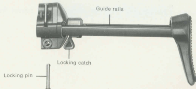
Fig. 15 Retractable butt stock
