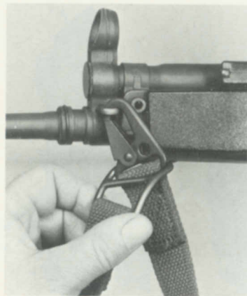
Fig. 41 Pulling the double loop over the carbine hook
