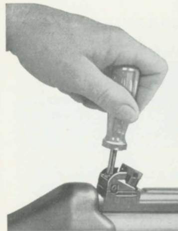
Fig. 39 Loosening the clamping screw
