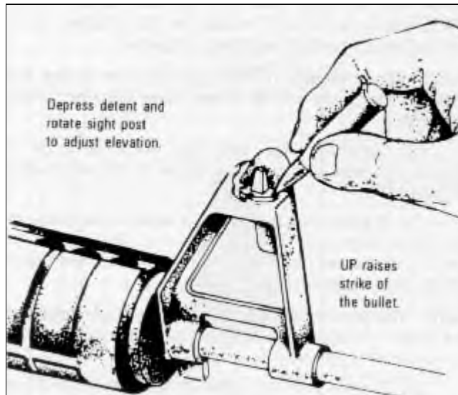
Figure 111. Depress detent.
