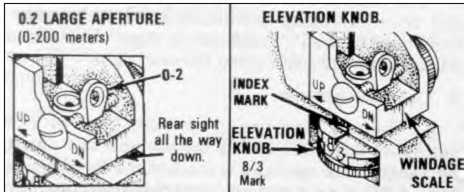
Figure 107. Rear sight.
