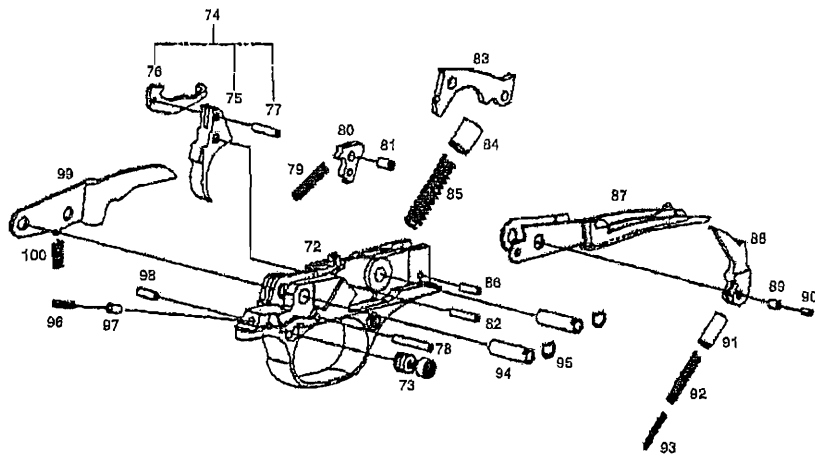
Figure 2: Trigger Plate Parts Assembly
