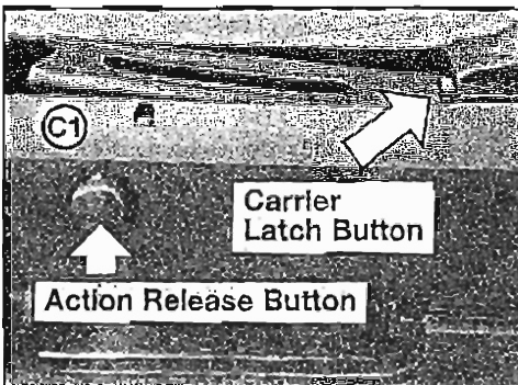
Action locked back properly
