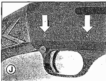
Gently tap out the front and rear trigger assembly pins with a punch
