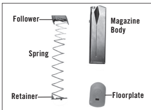
The magazine shown disassembled.
