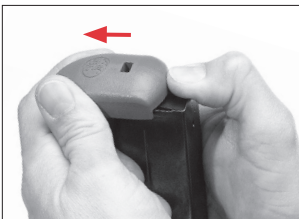
Slide the floorplate forward partially to secure the magazine spring.
