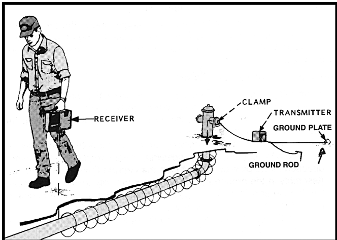
Figure 9. Conductive Trace
