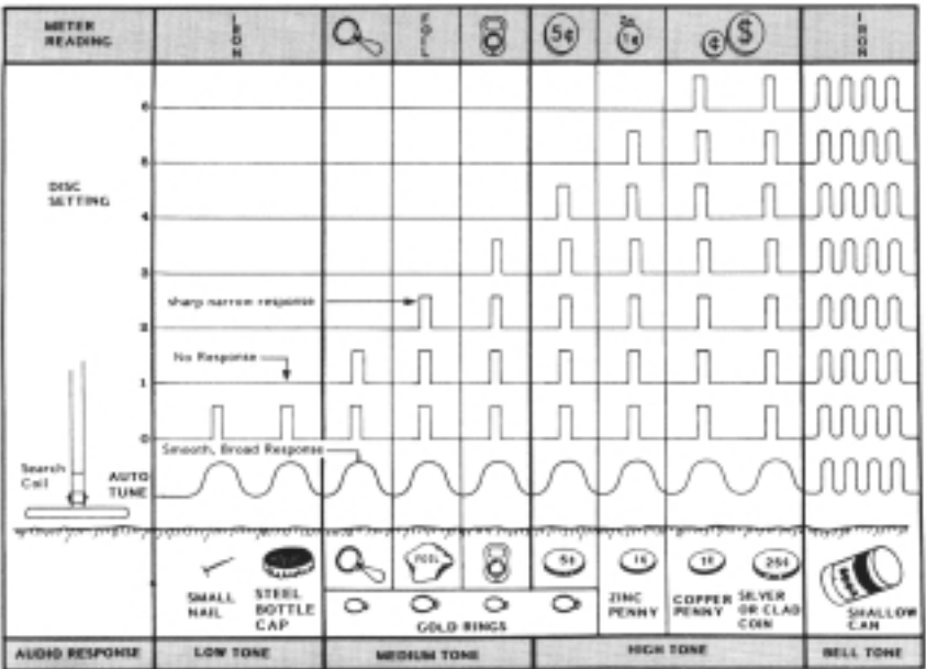
Figure 3. Typical 1266-X audio responses over 1 inch deep targets with search coil sweeping 1 to 2 inches above ground.
