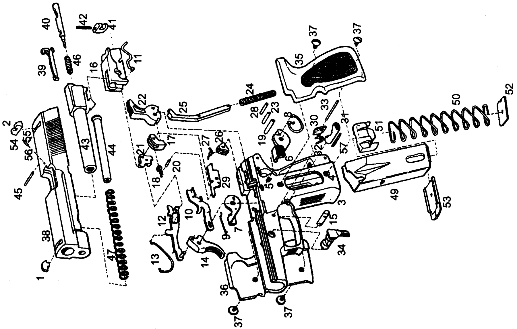
Fig. 15 EZ SERIES PISTOL PISTOL PARTS
