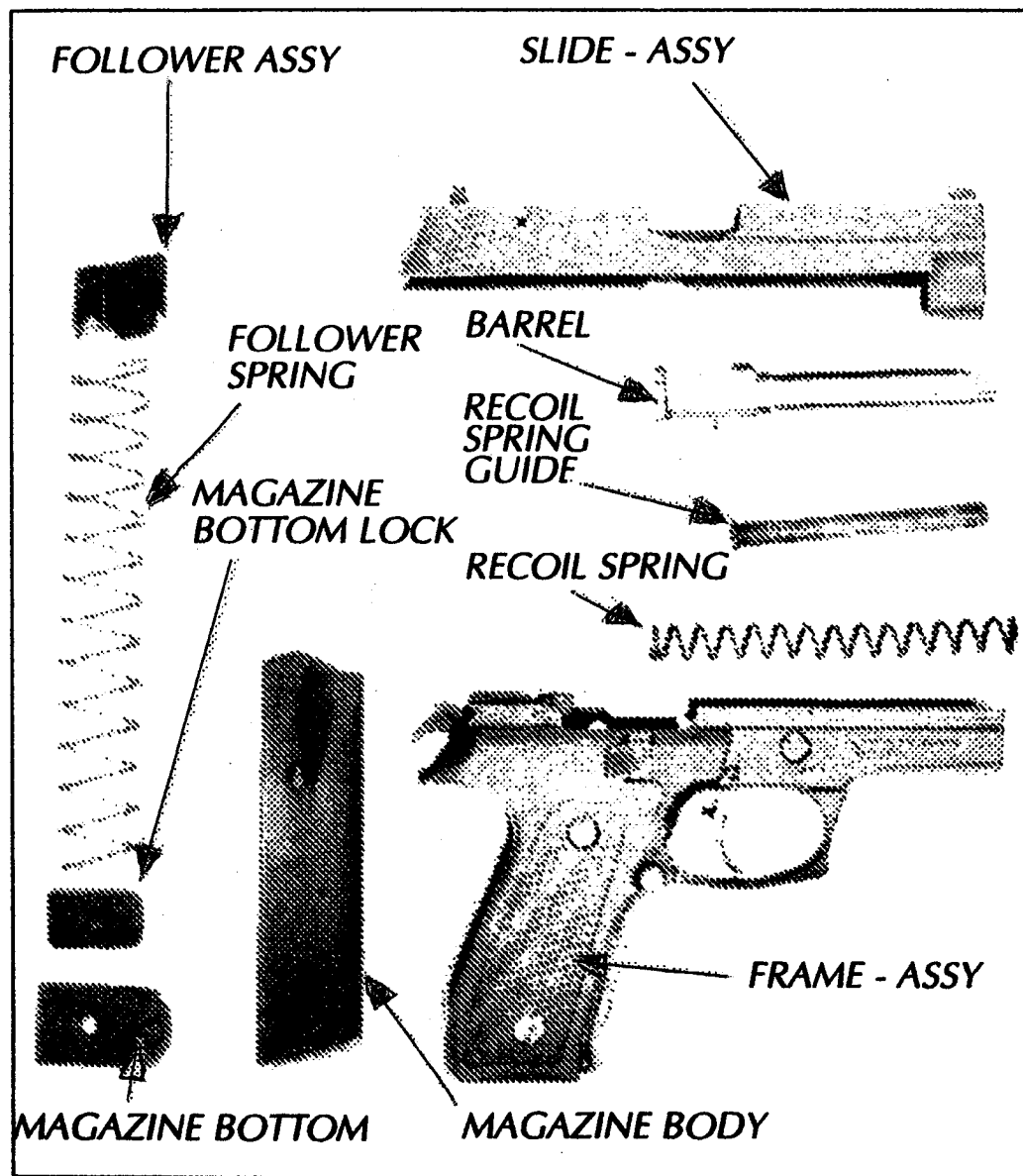
Fig. 14 STRIPPED PISTOL
