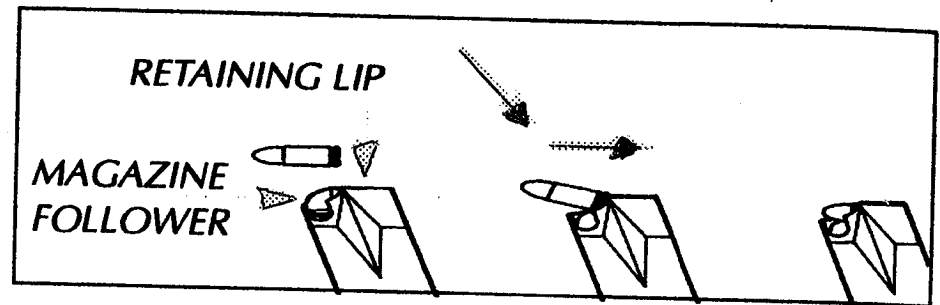
Fig. 6 MAGAZINE LOADING
