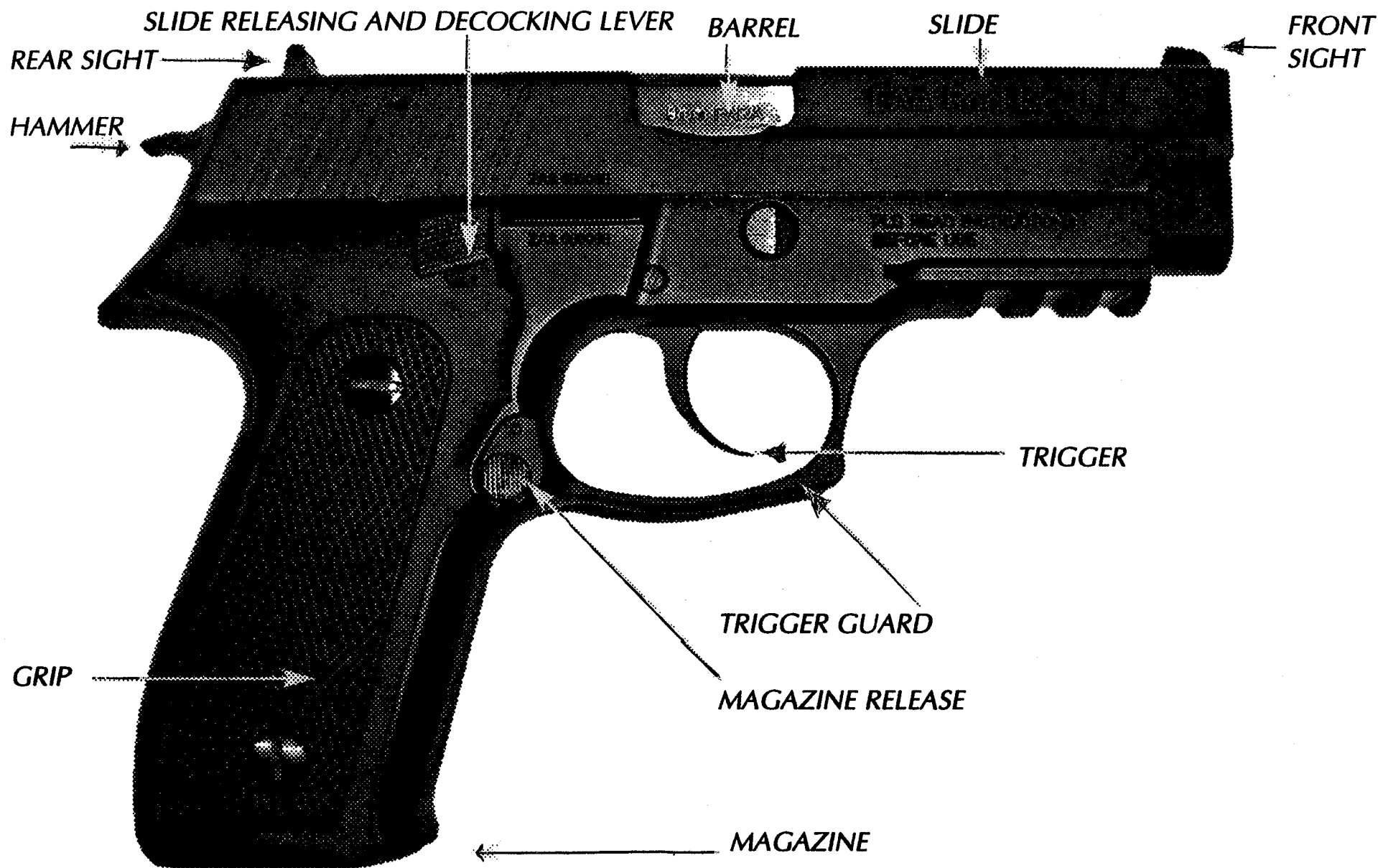
Fig. 1 EZ SERIES PISTOL - RIGHT SIDE
