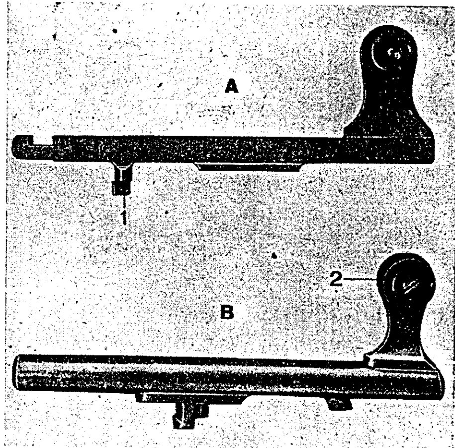
Figure 8 Cam Follower
