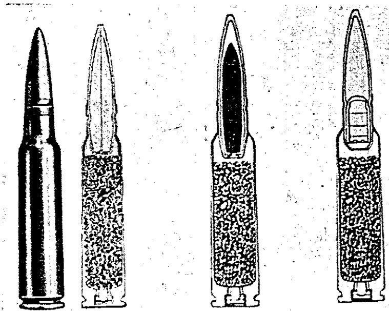
Common Rifle Cartridge 11
