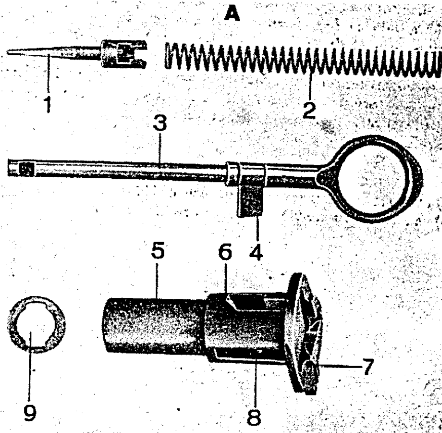
Fig. 11 Firing Mechanism
