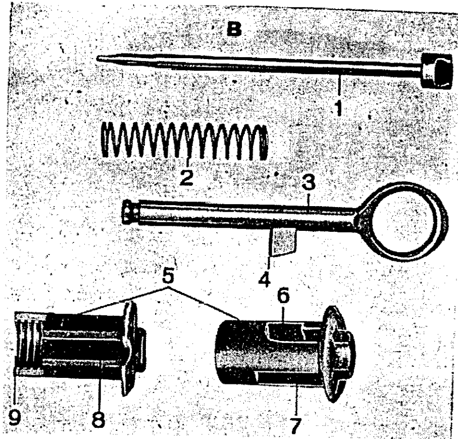
Fig. 12 Firing Mechanism
