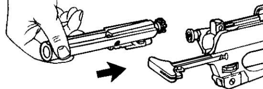
10.) Position Carrier Key in slotted bottom of Charging Handle. Slide in Bolt Carrier Group.
