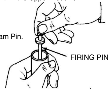
6.) Drop in and seat the Firing Pin.
