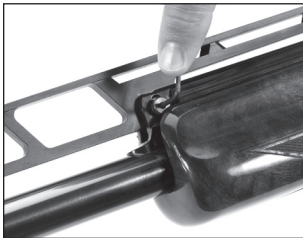
Loosen both screws at the rib pivot point.
