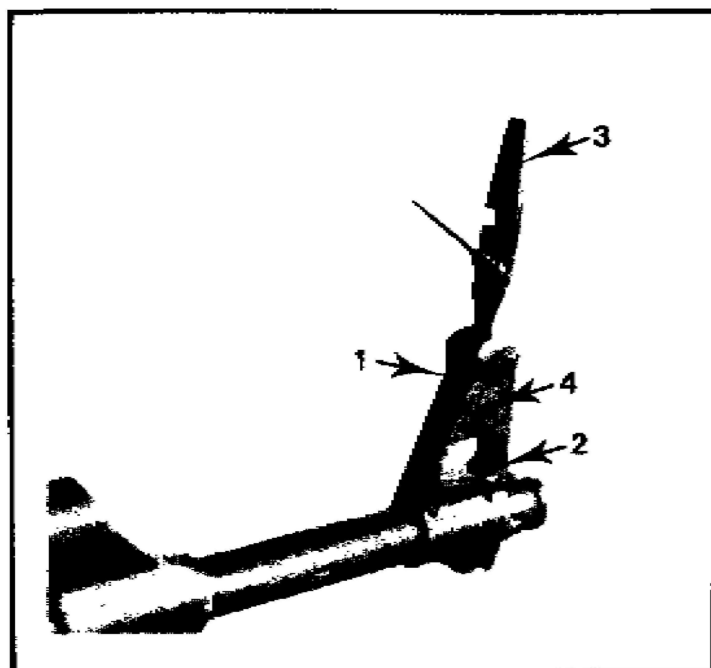
FIGURE 18. FRONT SIGHT
