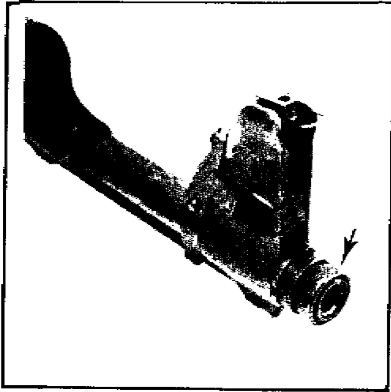
FIGURE 53. MUZZLE NUT
