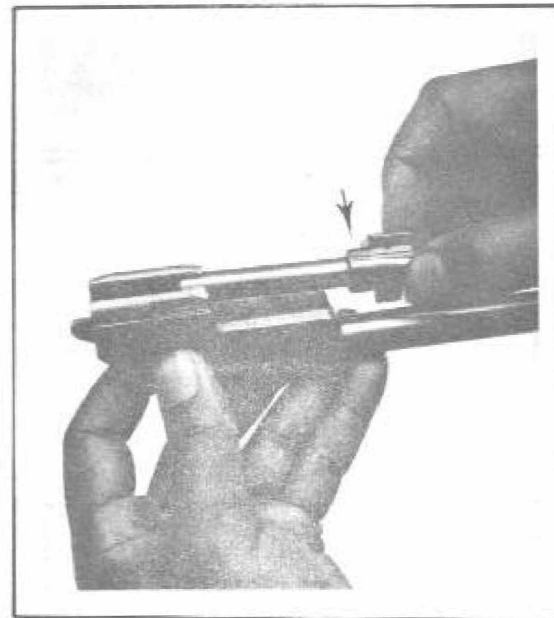
FIGURE 31. REMOVING BOLT
