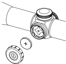
VX-R battery location
