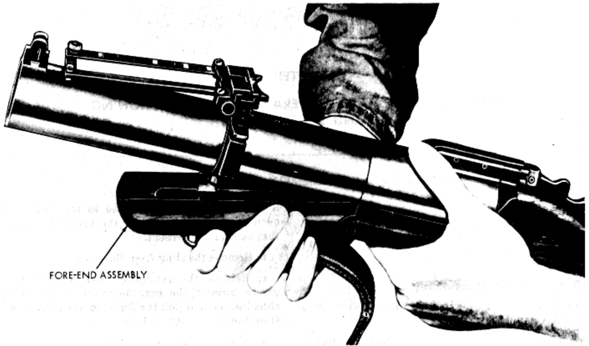
Figure 10-2. Removing or installing fore-end assembly.
