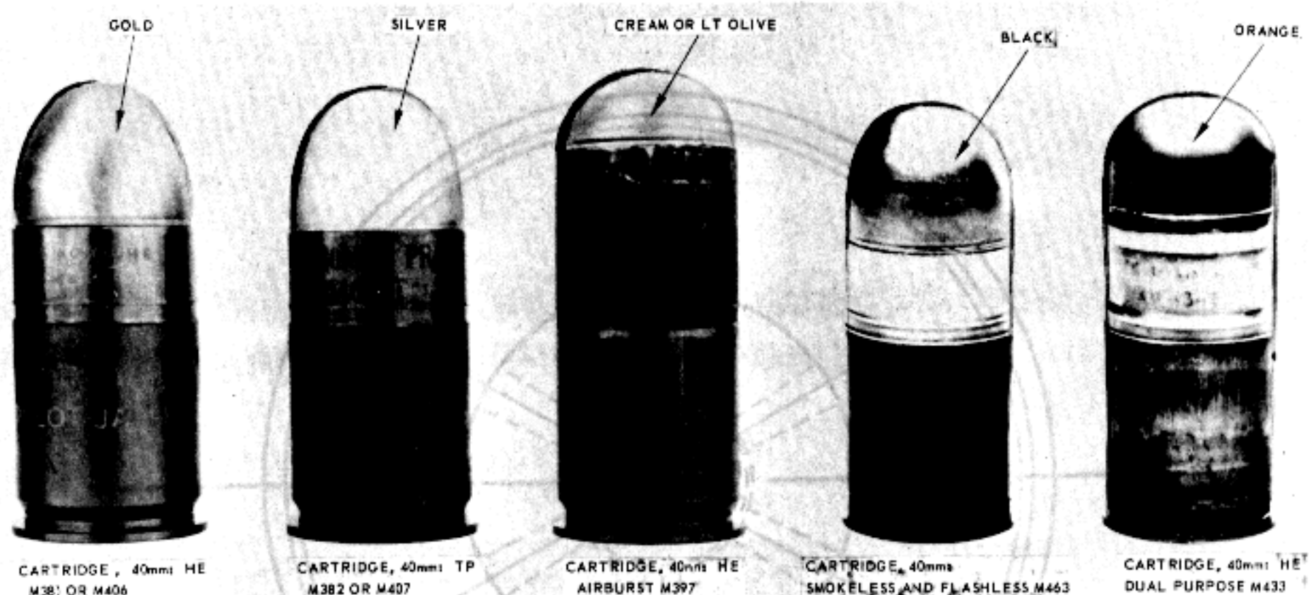
Figure 4-2. Some standard 40-mm cartridges available for use with the grenade launcher, M208.
