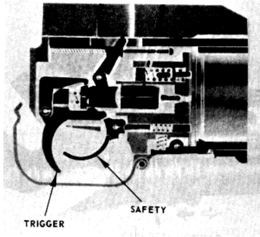
(2) In the safe position. Figure 2-2.—Continued.
