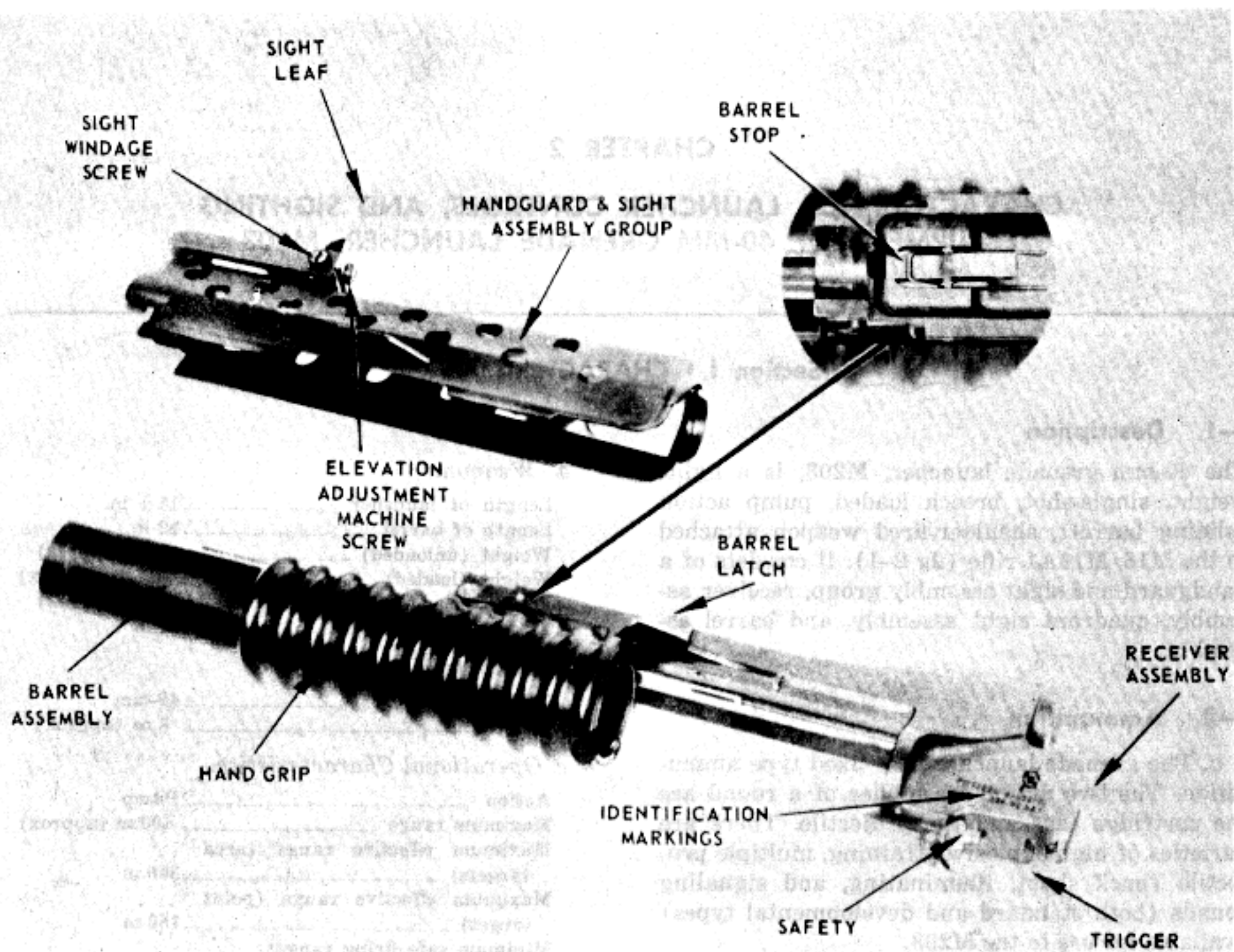
(2) Controls and identifications. Figure 2-1.—Continued.
