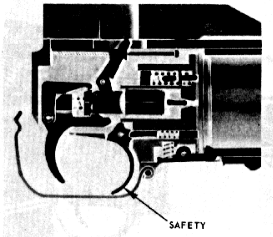
(1) In the firing position. Figure 2-2. Location of the safety.
