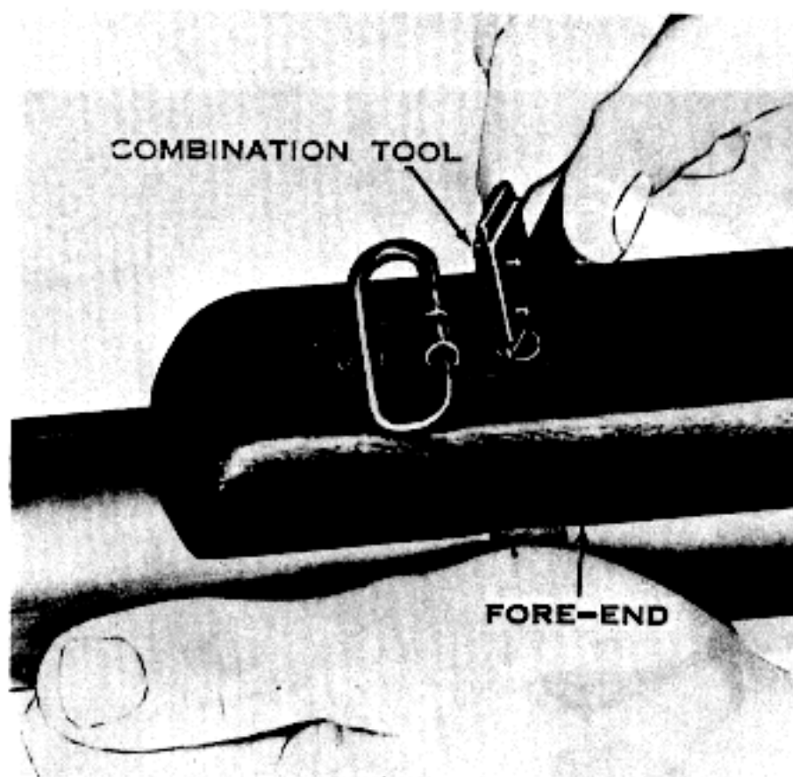
Figure 10-1. Removing or installing the retaining band screw.
