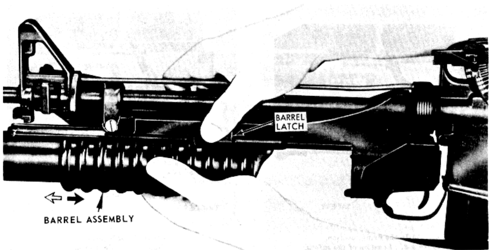
Figure 2-4. Operating the barrel latch.
