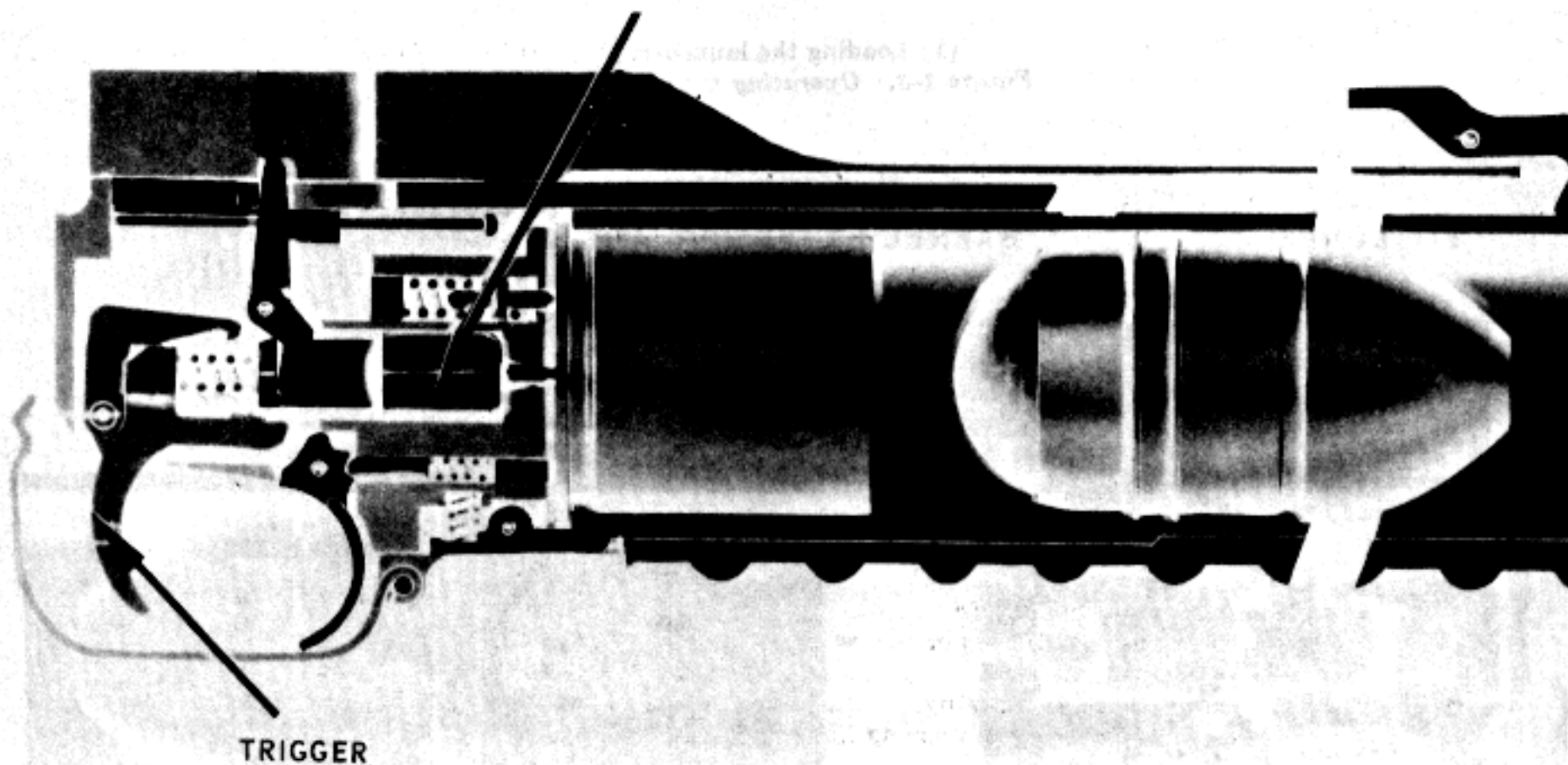
(4) Firing. Figure 3-3.—Continued.
