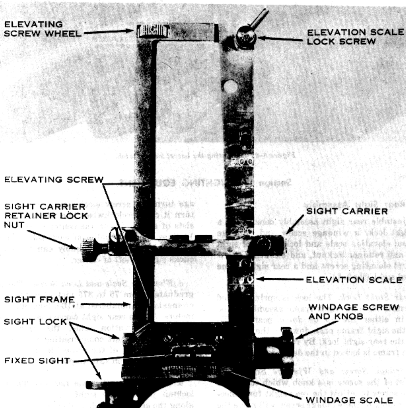
Figure 9-7. Rear sight assembly.
