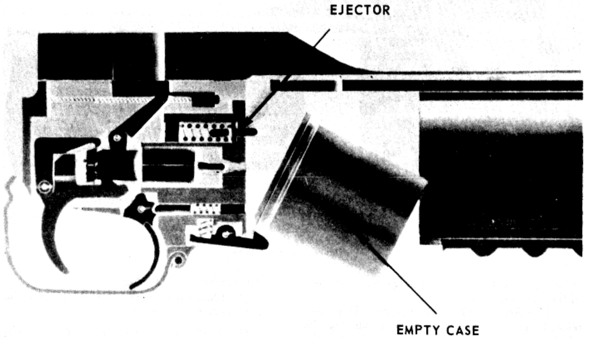
(4) Ejection. Figure 3-2.—Continued.
