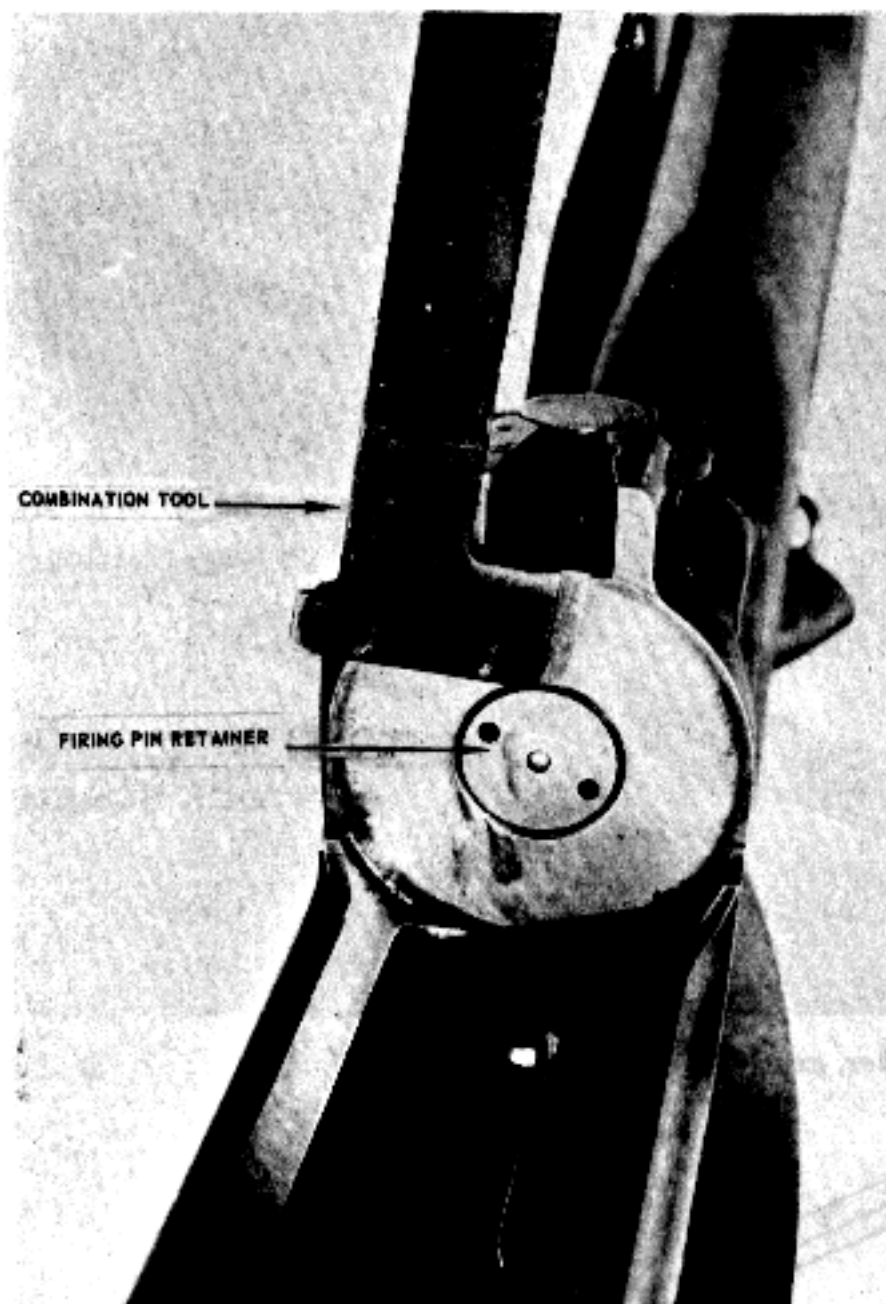
Figure 10-6. Position of firing pin retainer.
