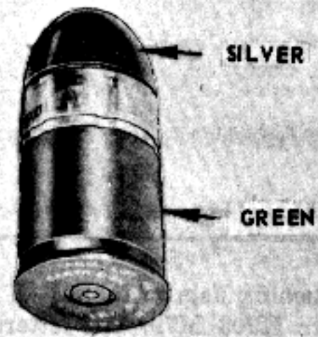
CARTRIDGE 40-mm TP M 382 OR M 407A1
