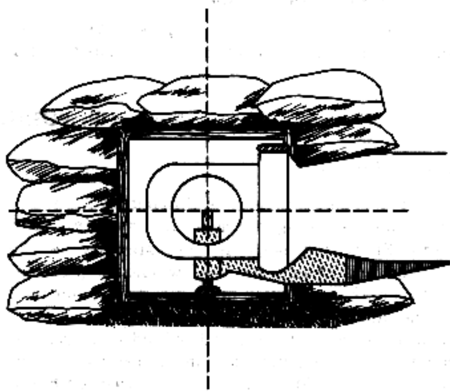
(2) With quadrant sight. Figure 6-1.—Continued.
