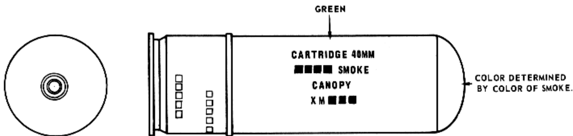
Figure B-9. 40-mm, red smoke cartridge XM675.
