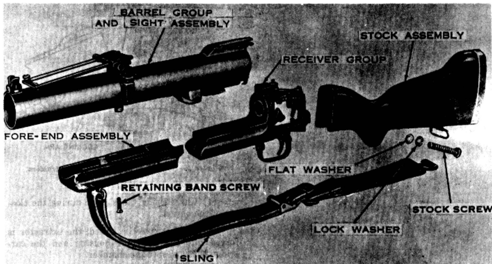
Figure 10-4. Grenade launcher, general disassembly.
