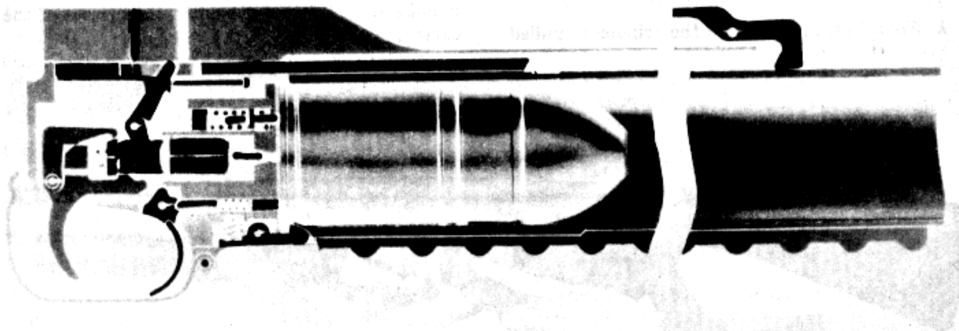
(3) Locking the barrel. Figure 3-3.—Continued.
