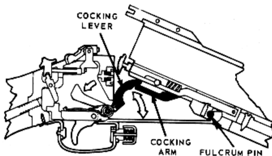
Figure 10-5. Assembling barrel group and receiver group.
