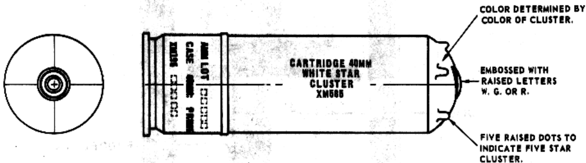
Figure B-5. 40-mm star parachute cartridge XM588, XM661, XM662, and XM695.
