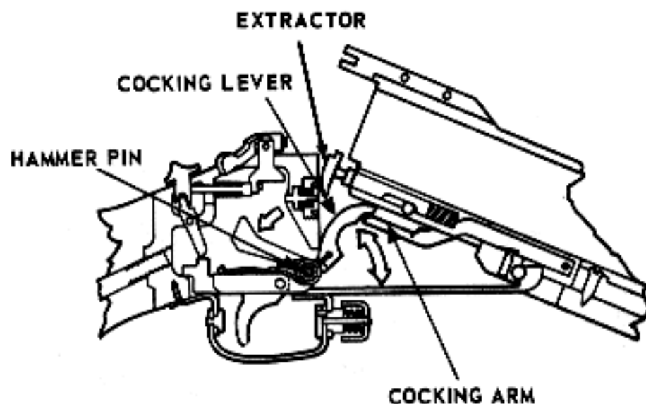
Figure 10-7. Unlocking, cocking, and extraction.
