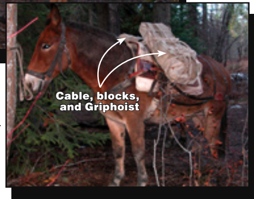
Figures 5a and 5b—The portable tripod can be transported into the backcountry by mules. One mule carries the tripod while another mule carries the block, Griphoist, and cables.
