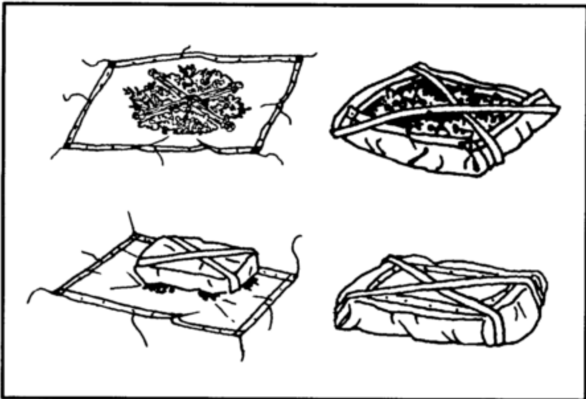
Figure 17-4. Brush raft.
