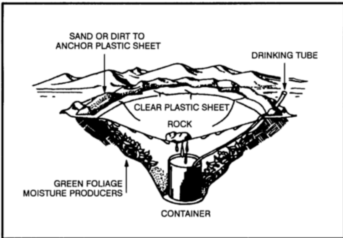
Figure 6-7. Belowground still.
