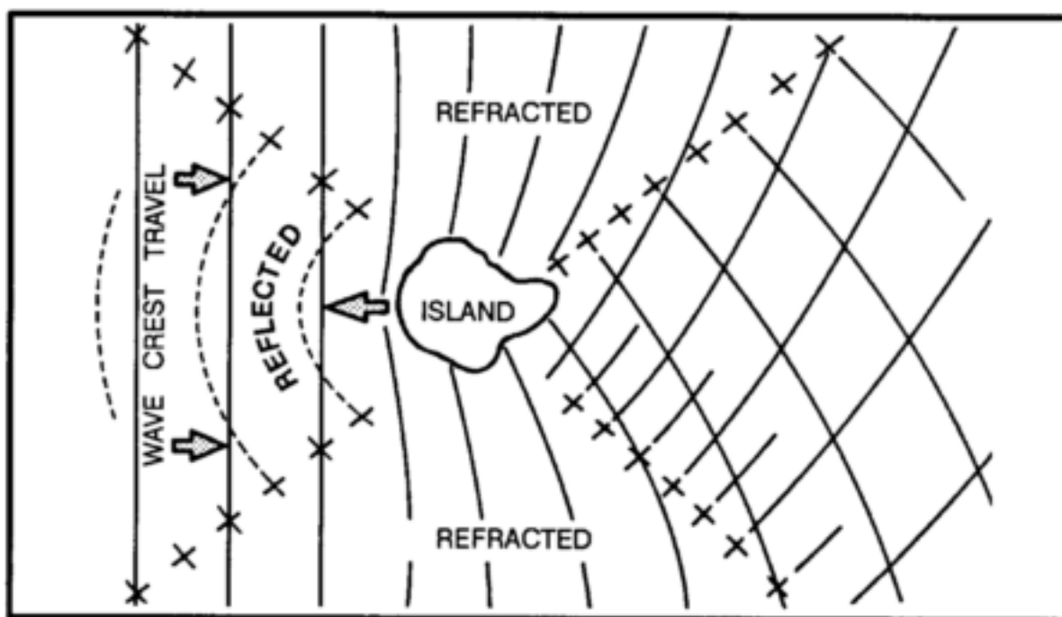
Figure 16-20. Wave patterns about an island.
