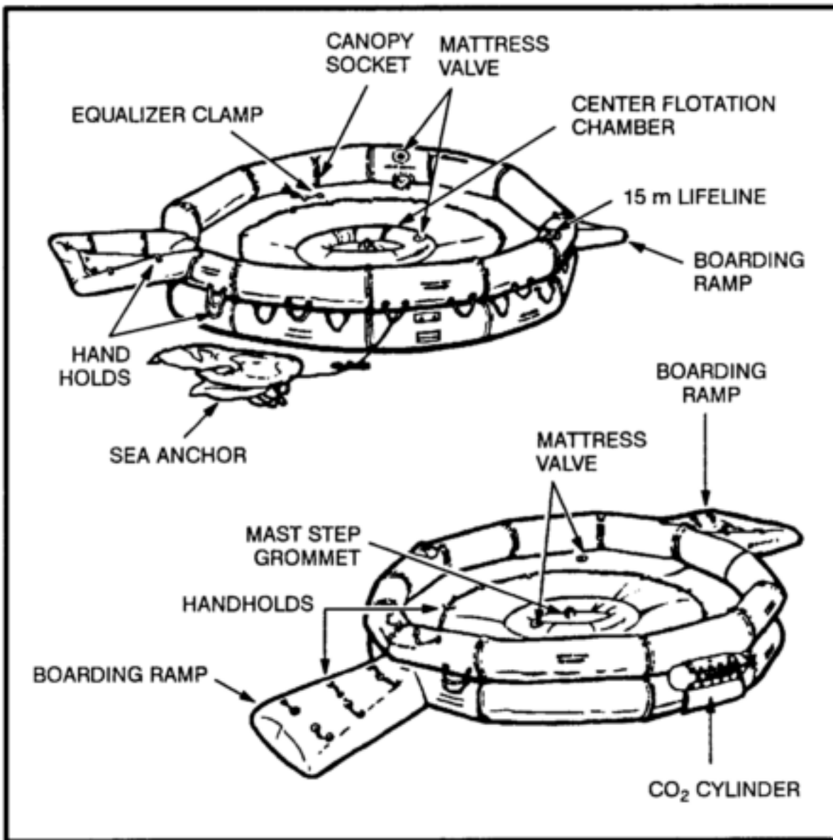
Figure 16-15. Twenty-man raft.
