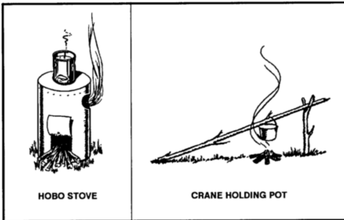
Figure 15-7. Cooking fire/stove.
