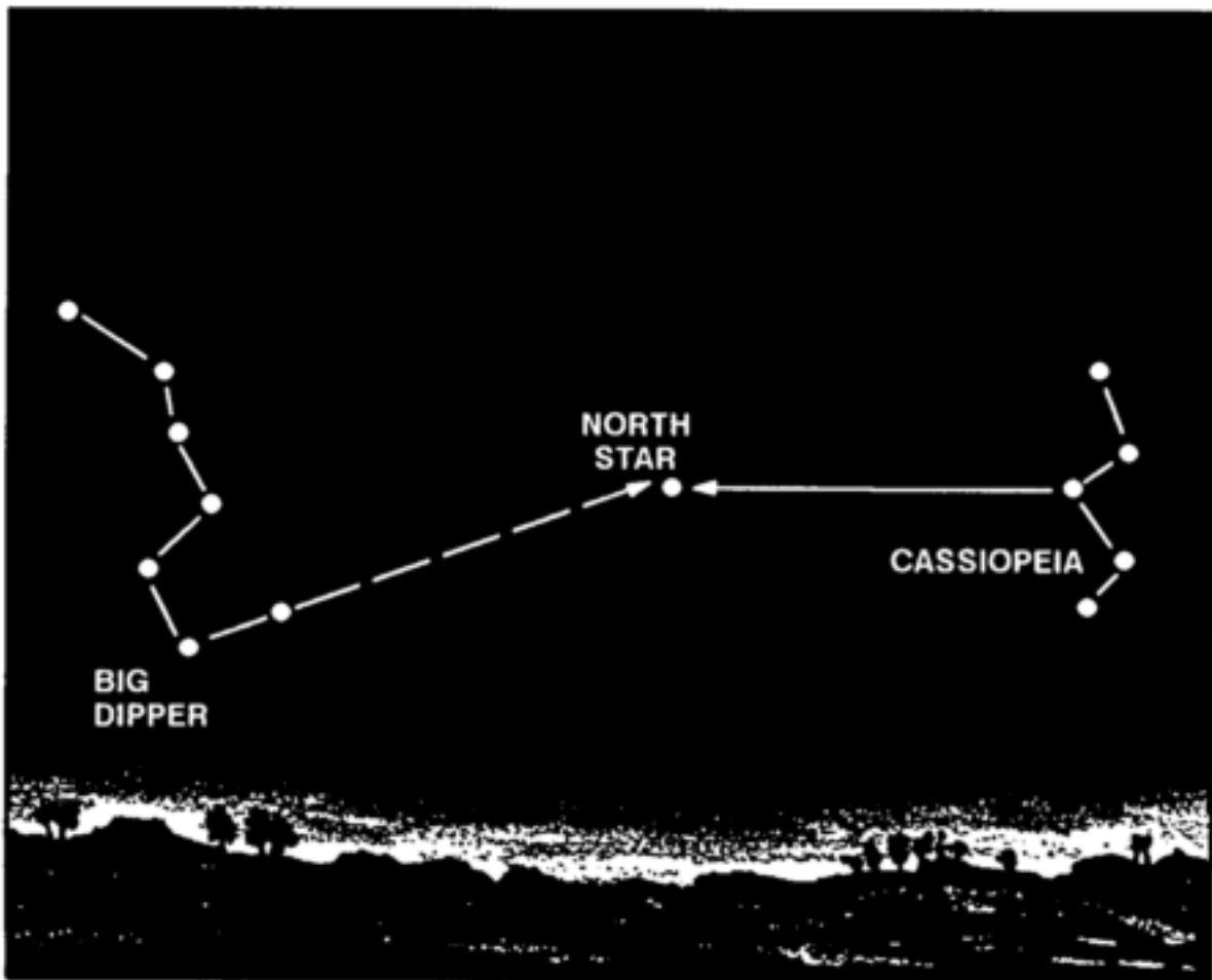
Figure 18-3. The Big Dipper and Cassiopeia.
