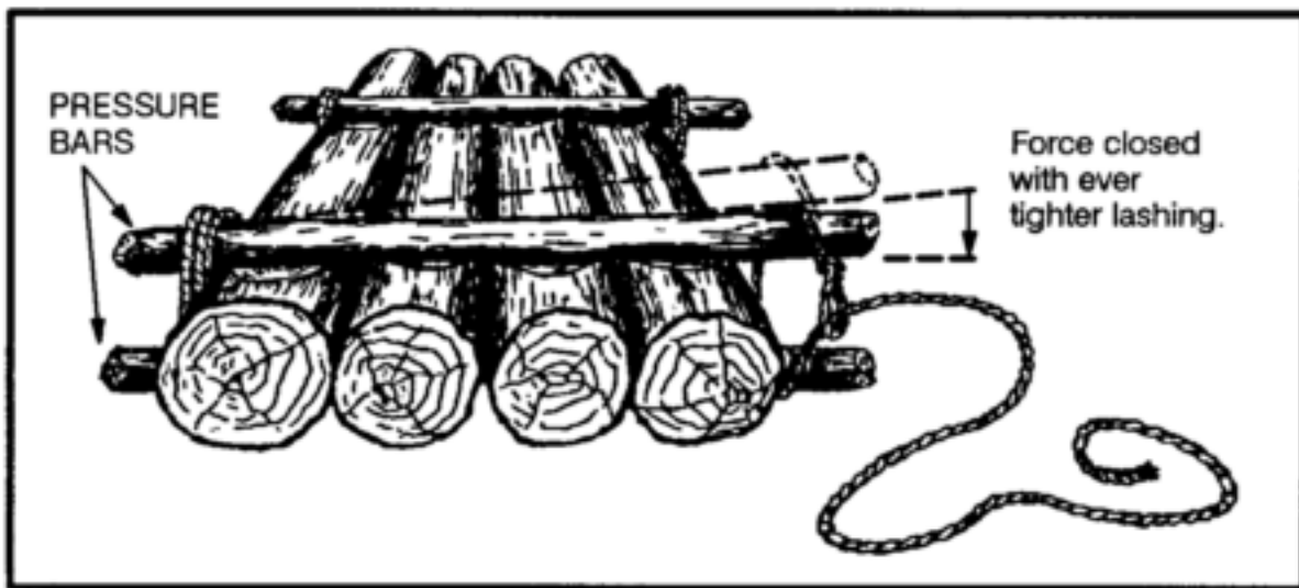
Figure 17-7. Use of pressure bars.
