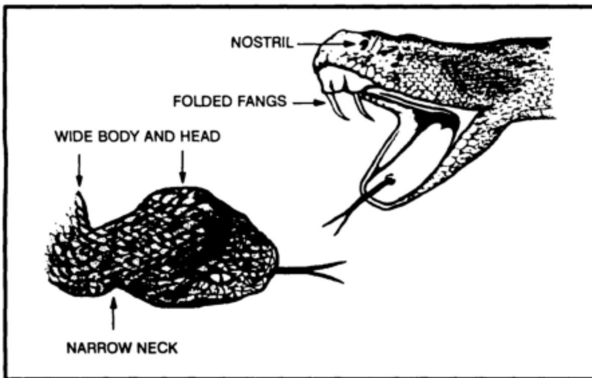
Figure E-3. Positive identification of vipers.
