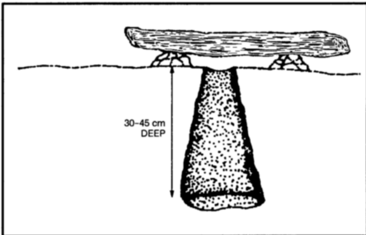
Figure 8-16. Bottle trap.
