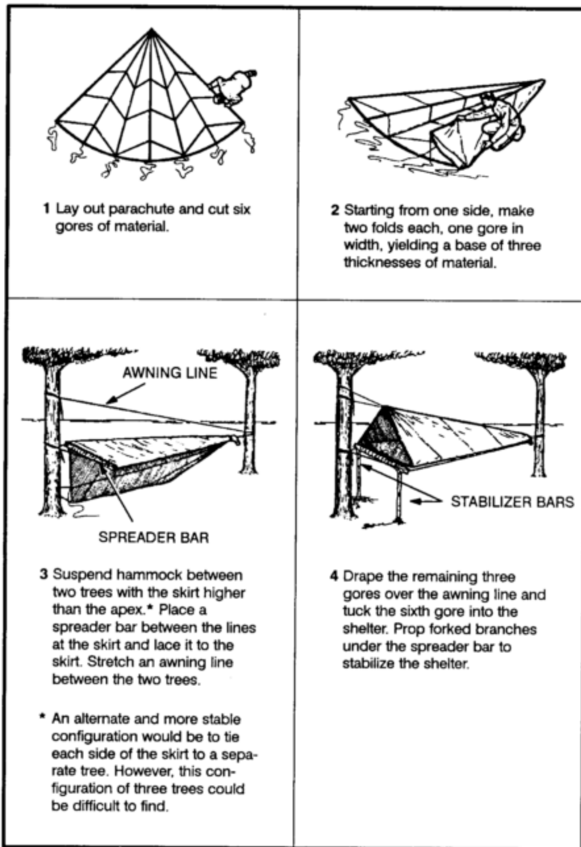
Figure 5-8. Parachute hammock.
