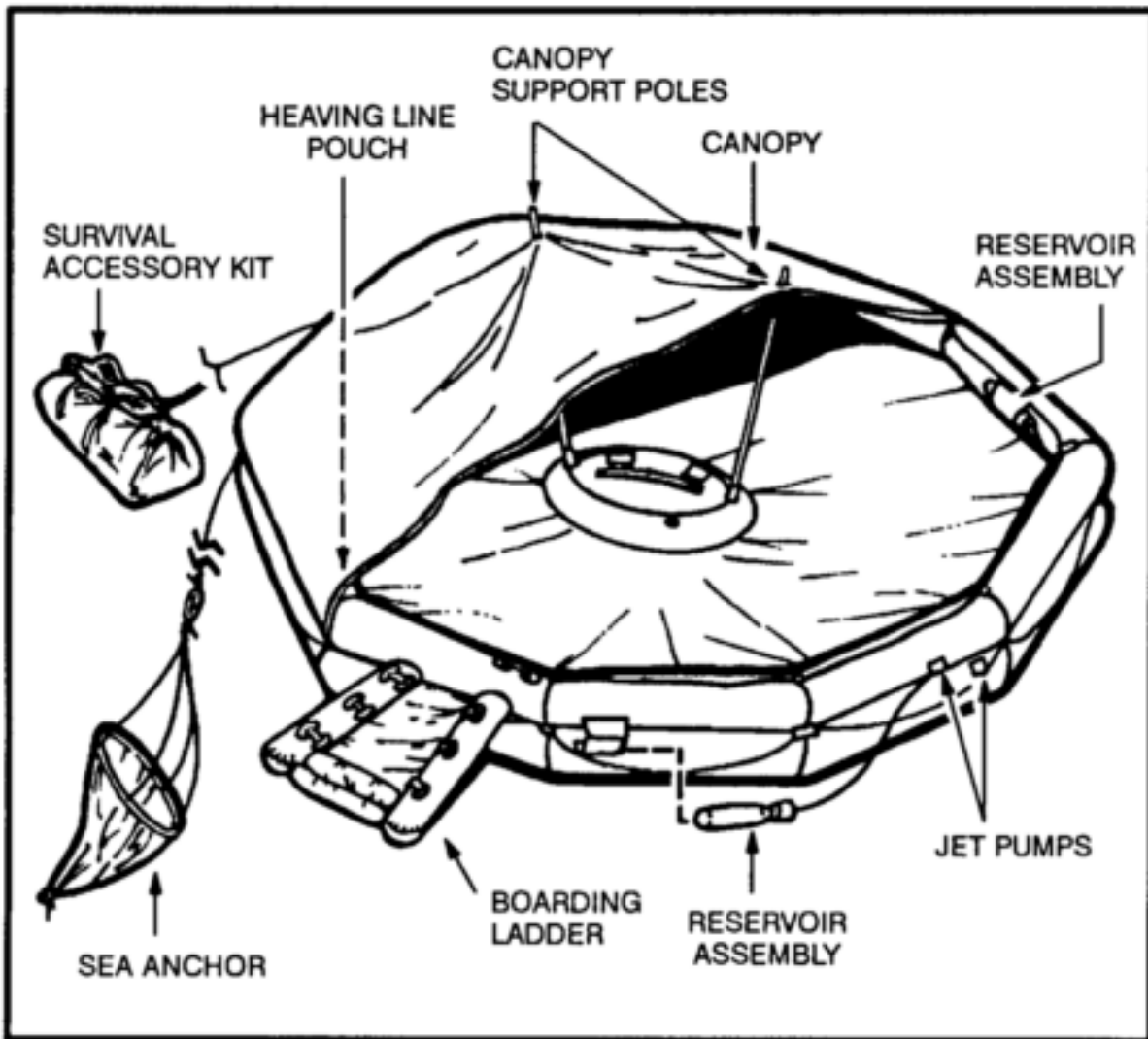
Figure 16-16. Twenty-five-man raft.
