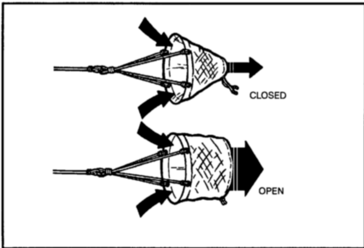
Figure 16-5. Sea anchor.
