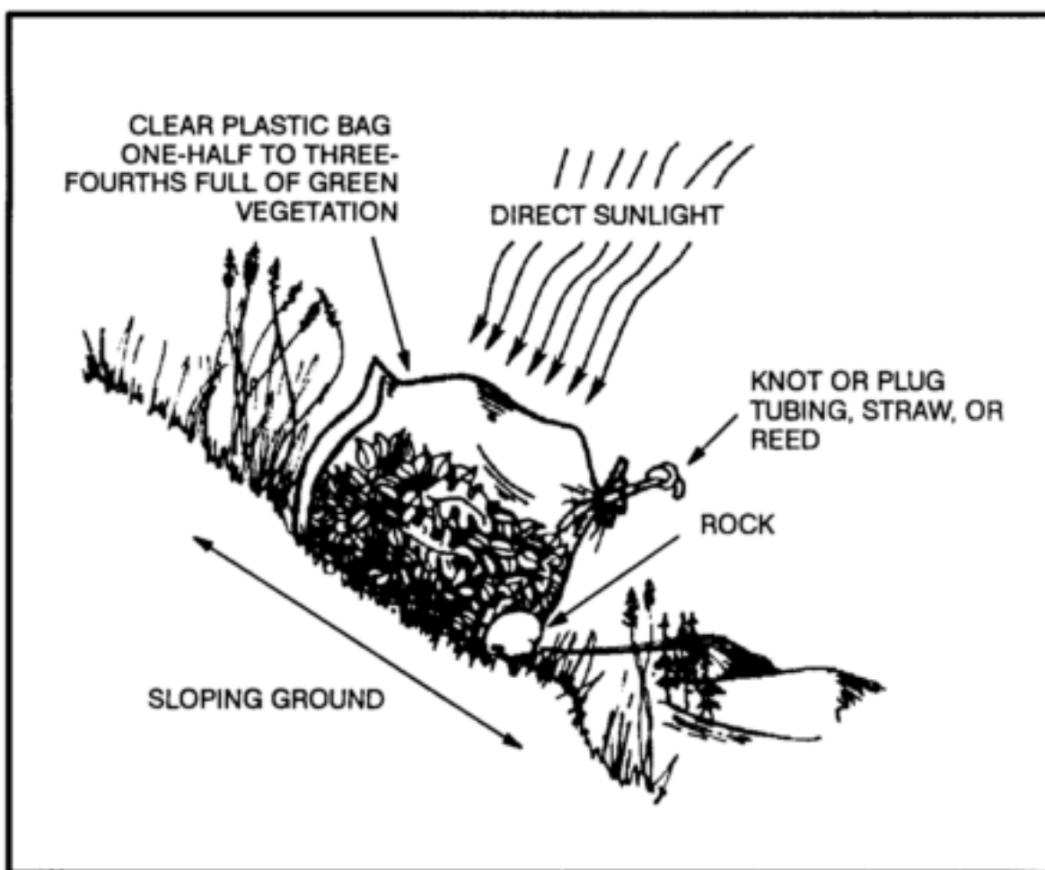
Figure 6-6. Aboveground solar water still.
