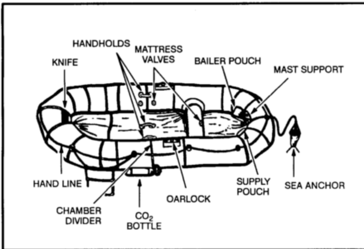
Figure 16-12. Seven-man raft.
