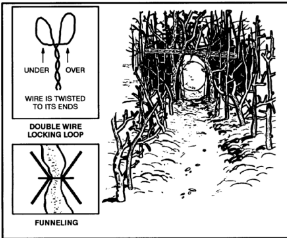
Figure 8-6. Drag noose.
