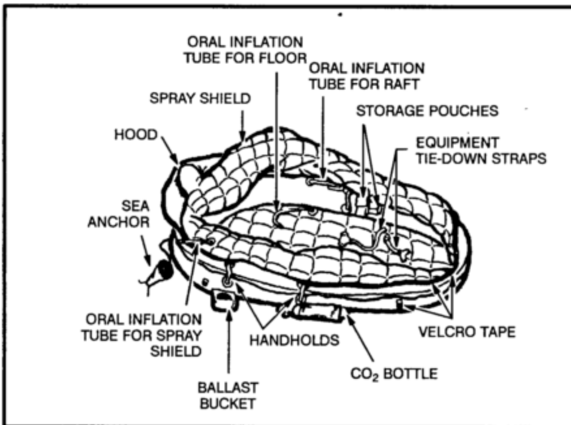
Figure 16-8. One-man raft with spray shield.
