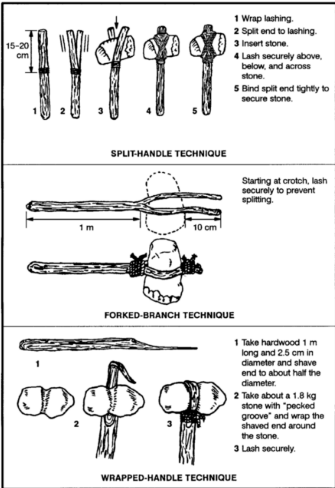
Figure 12-1. Lashing clubs.
