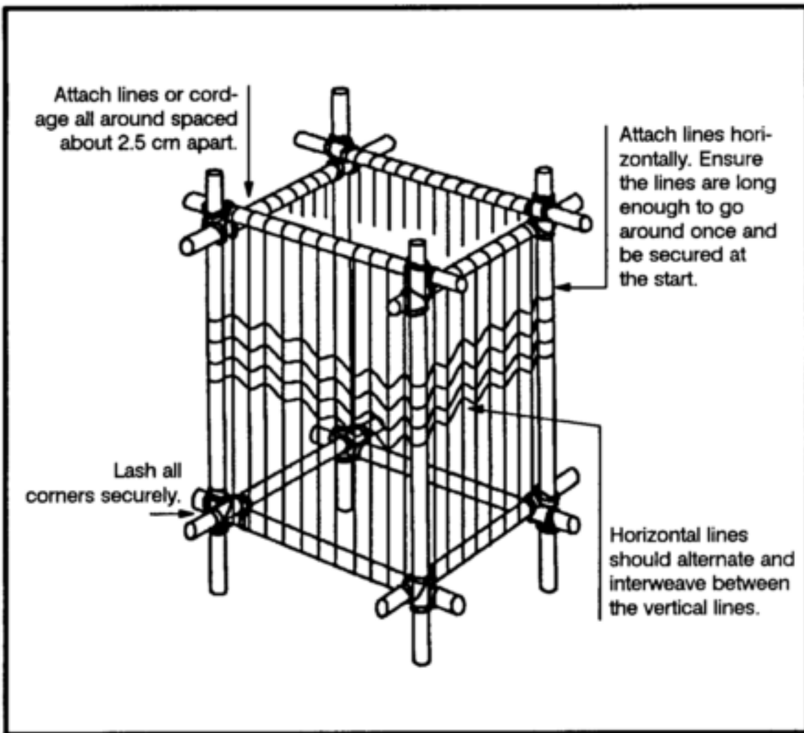
Figure 12-10. Square pack.
