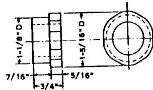
DETAIL OF END NUT MAKE FROM STANDARD 7/8" HEXAGONAL NUT
