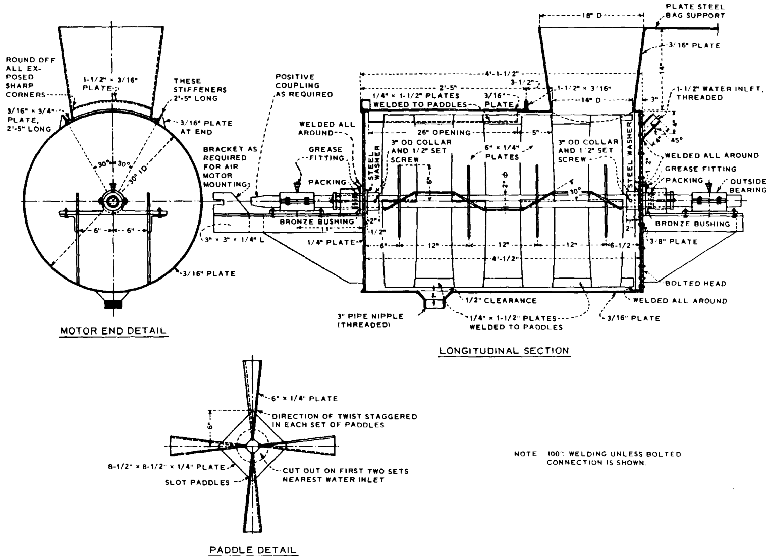
Figure 6-10. Horizontal drum grout mixer, 8-cubic-foot capacity
