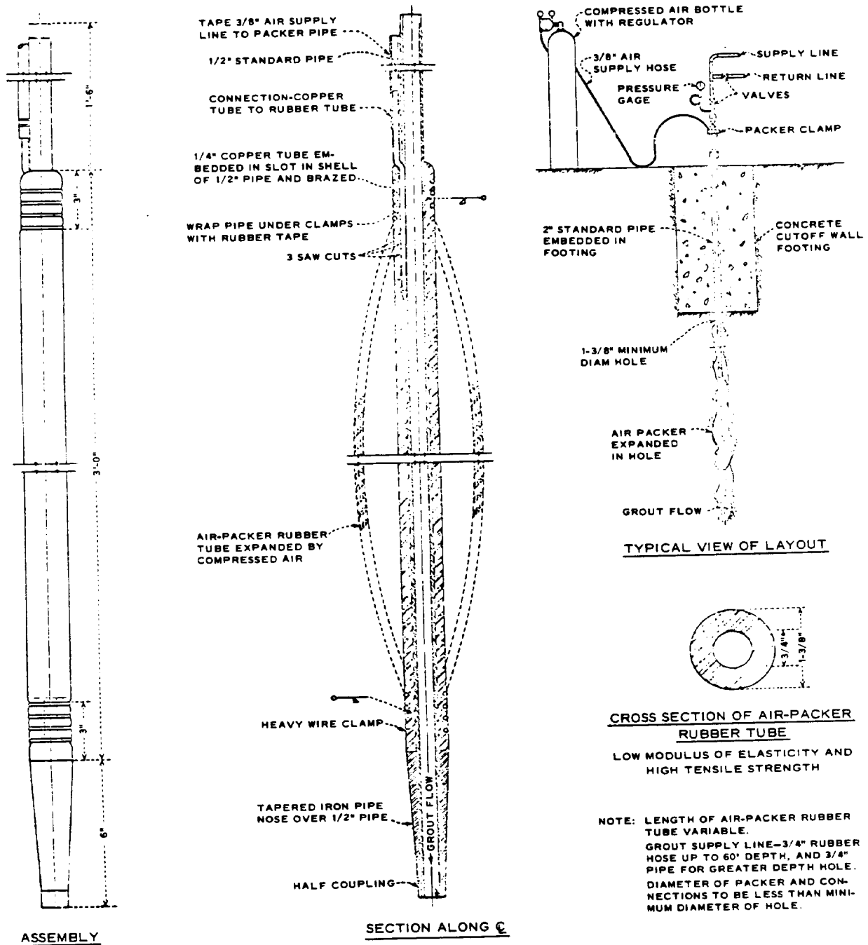
Figure 6-17. Air packer
