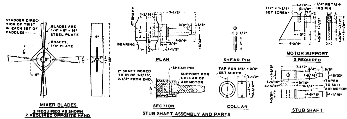
Figure 6-11. Horizontal drum grout mixer, 27-cubic-foot capacity
