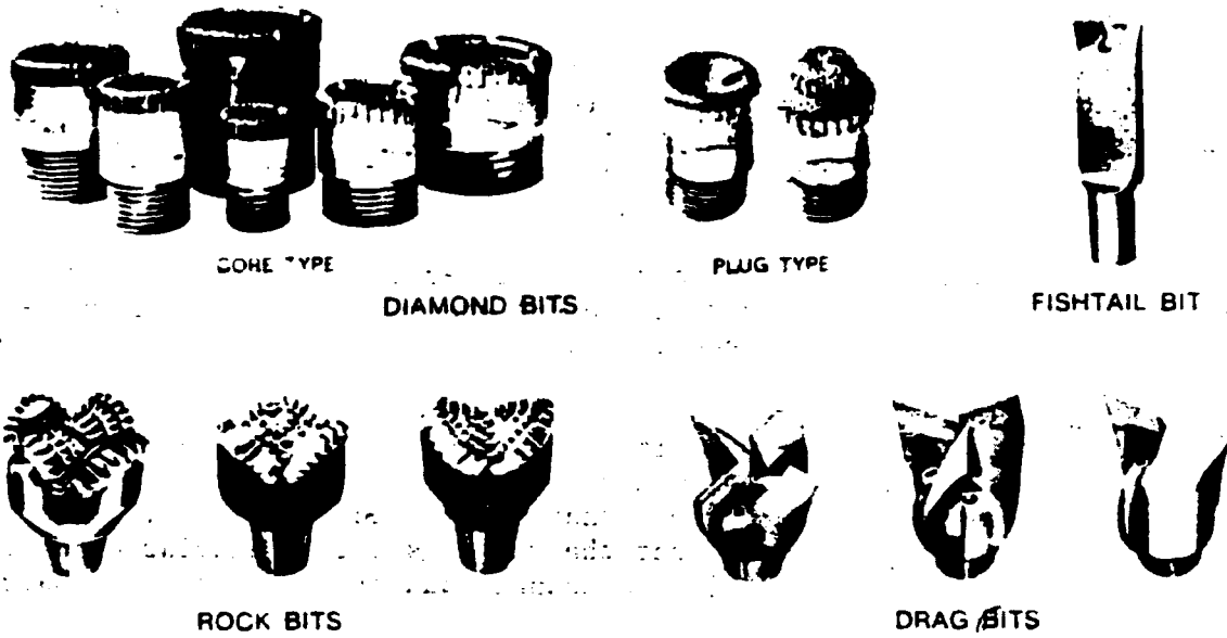
Figure 6-6. Drill bits
