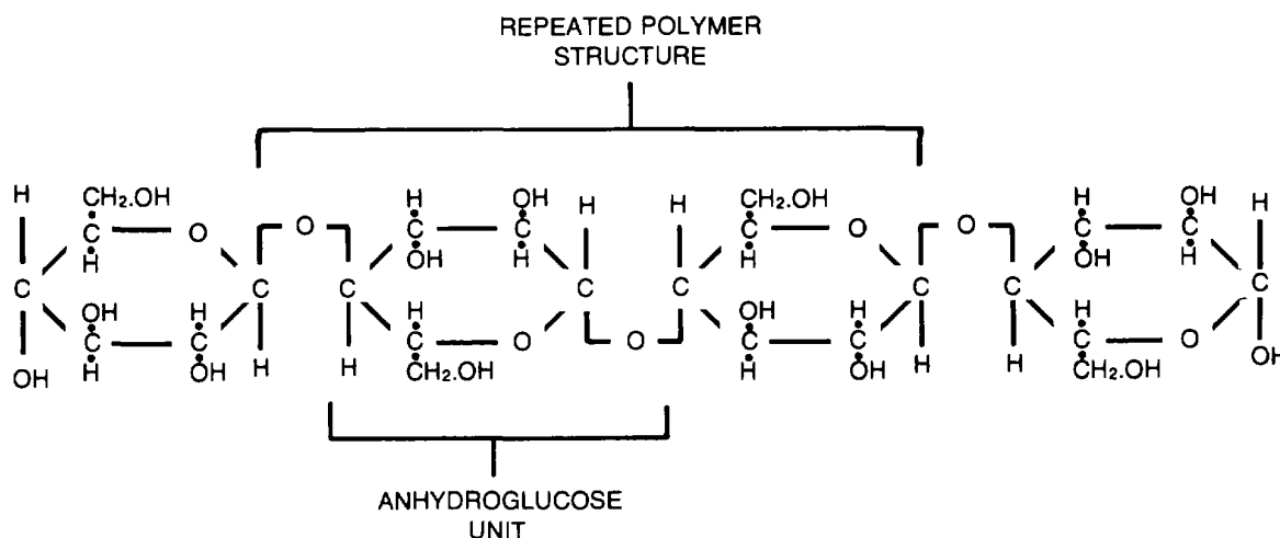
Figure 8-3. Cellulose.
