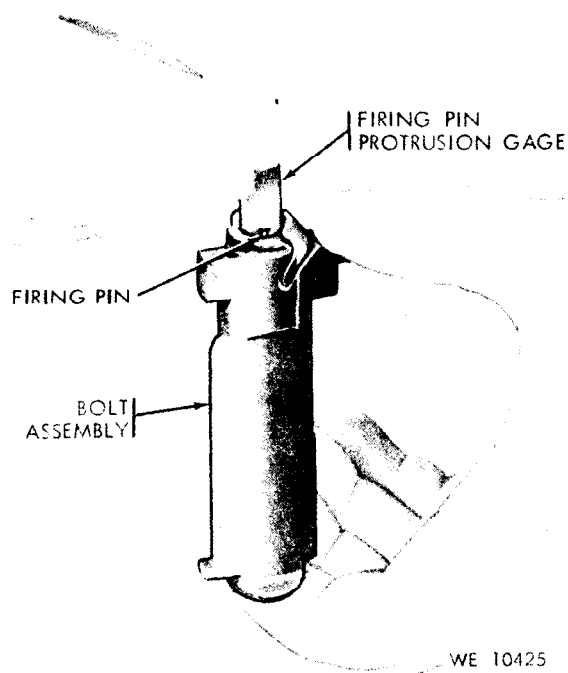
Figure 5-17. Gaging firing pin protrusion.
