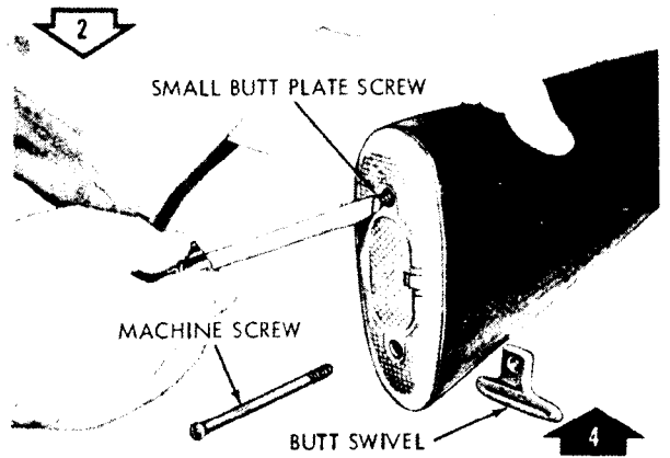
DISASSEMBLE/ASSEMBLE SMALL BUTT PLATE SCREW.
