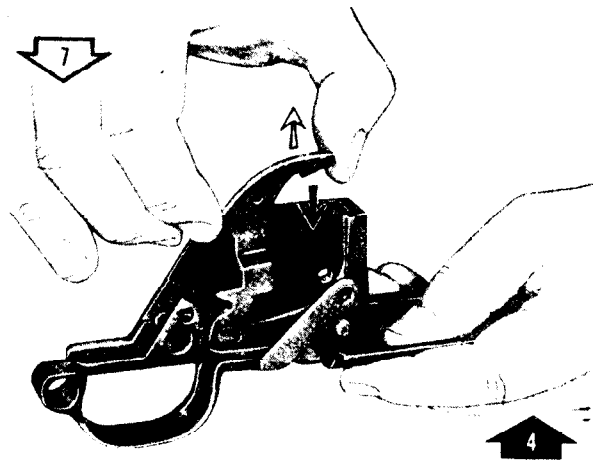
DISASSEMBLE/ASSEMBLE SAFETY.
