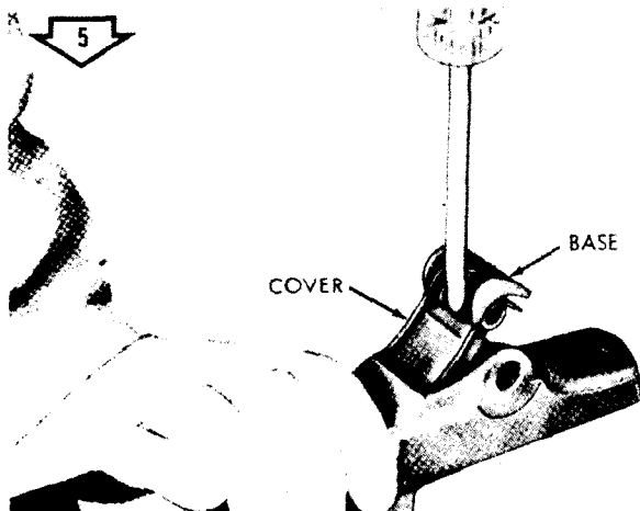
5 SEPARATE REAR SIGHT COVER FROM BASE. COVER BASE
