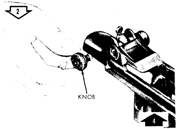
2 DISASSEMBLE/ASSEMBLE WINDAGE KNOB. 4
