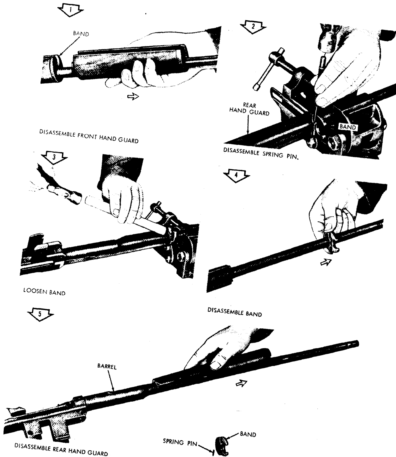
Figure 5-24. Disassembly of gun hand guard group.
