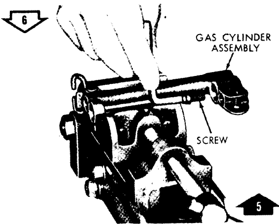
DISASSEMBLE/ASSEMBLE SOCKET HEAD SCREW.
