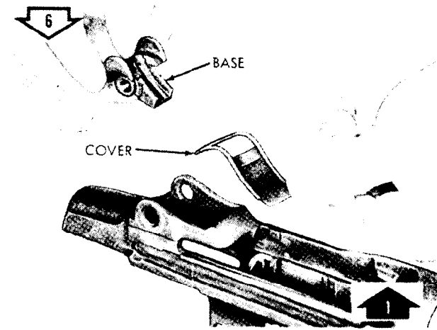
6 DISASSEMBLE/ASSEMBLE REAR SIGHT COVER AND BASE. COVER BASE 1
