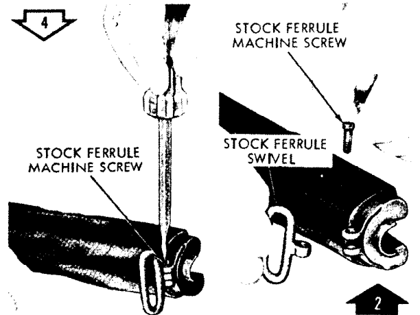
DISASSEMBLE/ASSEMBLE STOCK FERRULE MACHINE SCREW AND STOCK FERRULE SWIVEL.
