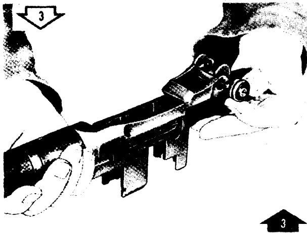
3 DISASSEMBLE/ASSEMBLE ELEVATING PINION. 3
