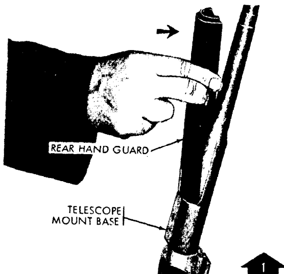
ASSEMBLE REAR HAND GUARD ON MID RIFLE.
