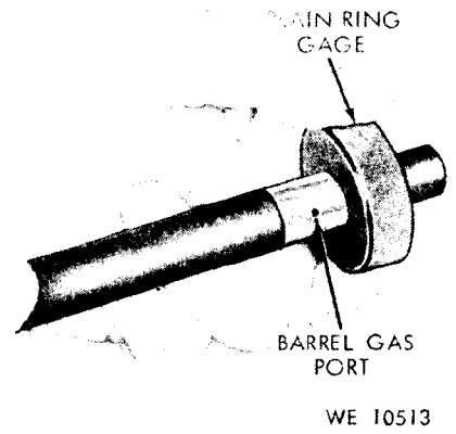
Figure 5-32. Gaging diameter of barrel at gas port.
