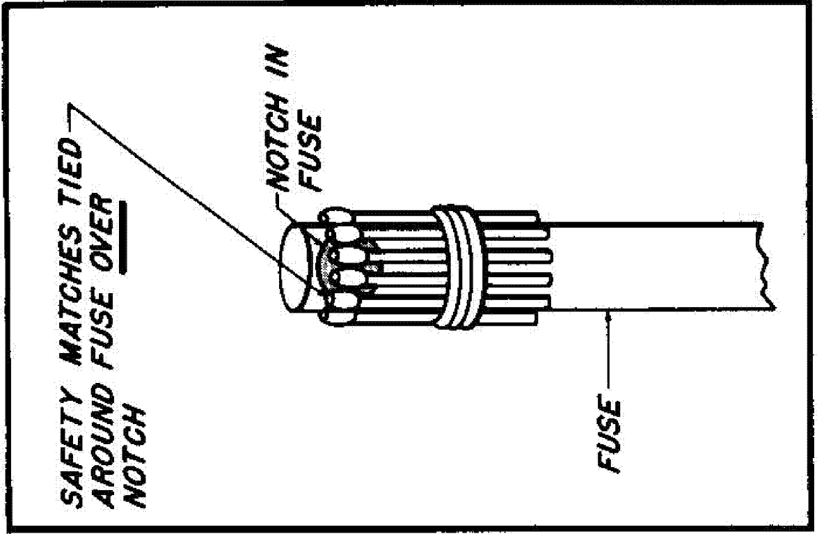
Fig. 59 — Time Fuse Fire Starter
