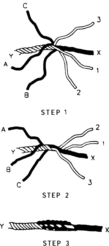
Figure 15-3. Making a short splice
