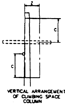
DETAIL-10
