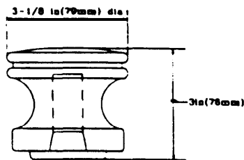
SPOOL CLASS 53-2
