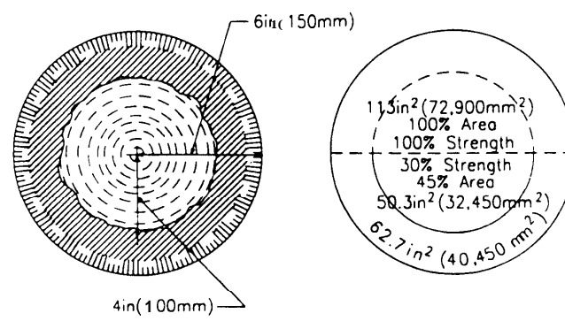
Decay has reduced 12-inch (300 millimeter) pole to 8-inch (200 millimeter) pole with only 45% of cross section (load supporting ability) and 30% of strength (resistance of bending) remaining
