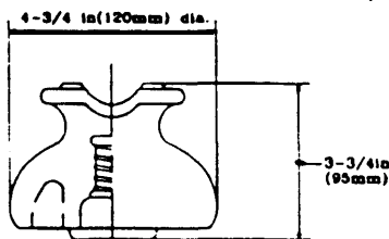
PIN, CLASS 55-3
