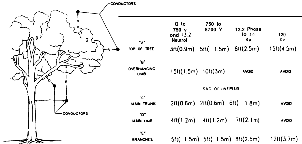
Figure 4-24. Recommended minimum clearances for tree trimming
