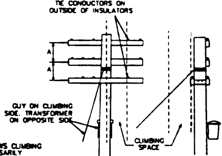
DETAIL-14
