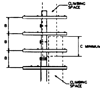
DETAIL-11
