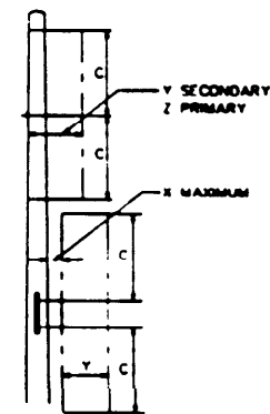
VERTICAL DIMENSIONS OF CLIMBING SPACE COLUMN
