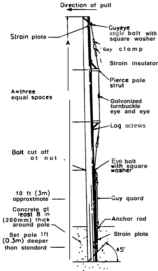
Figure 4-23. Self-supporting, hog-guyed pole
