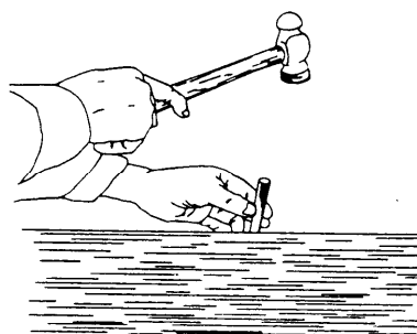
Figure 4-6. Sealing a test hole with a treated wooden plug
