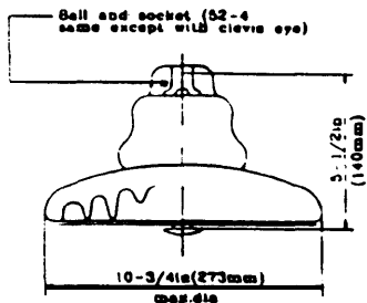
SUSPENSION, CLASS 52-3
