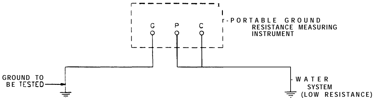
Figure 10-1. Direct-reference or two-point ground test
