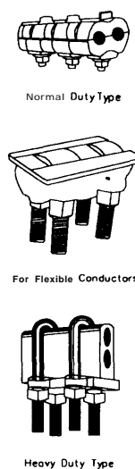
Figure 4-15. Clamp connectors (Courtesy of BURNDY Electrical)
