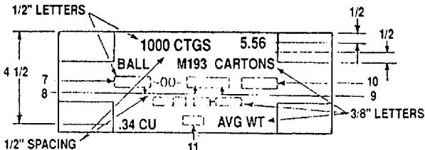
MARKING ON SIDE OF BOX (2 PLACES)
