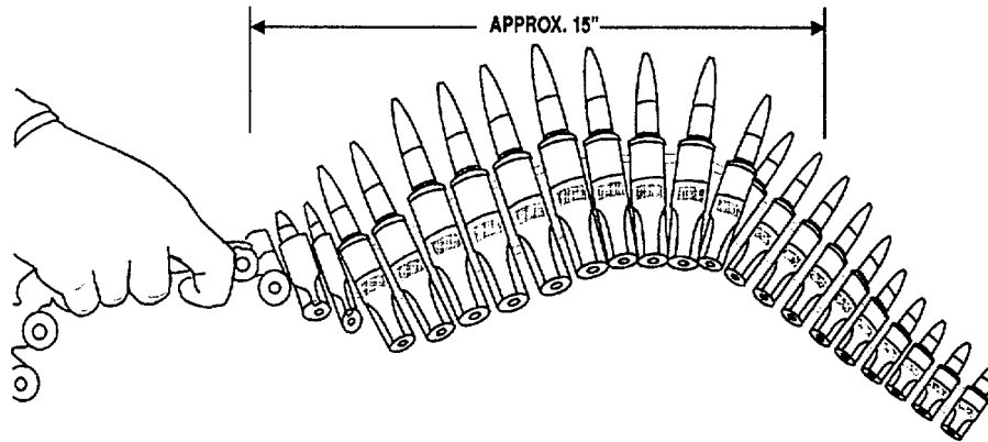
Figure 3-1. Twist inspection.
