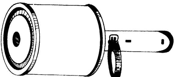
Figure 4-16. Soviet BPC-40 hand grenade.
