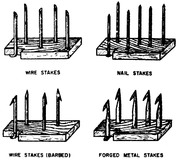
Figure 4-41. Barbed spike plates.
