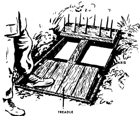
Figure 4-49. Pivoted spike board.
