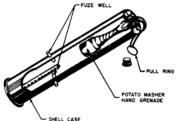
Figure 2-27. Shell case mine.
