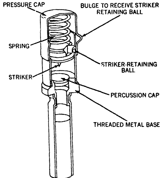
Figure 3-3. Soviet pressure fuze MV-6.
