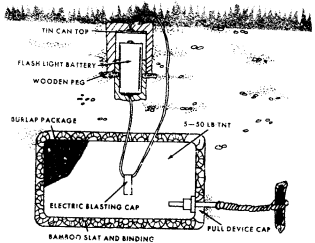
Figure 2-10. Typical locally fabricated VC mine (electrical detonation).
