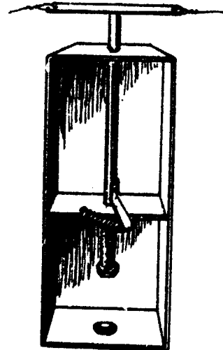
Figure 3-12. Viet Cong pressure/pull firing device.
