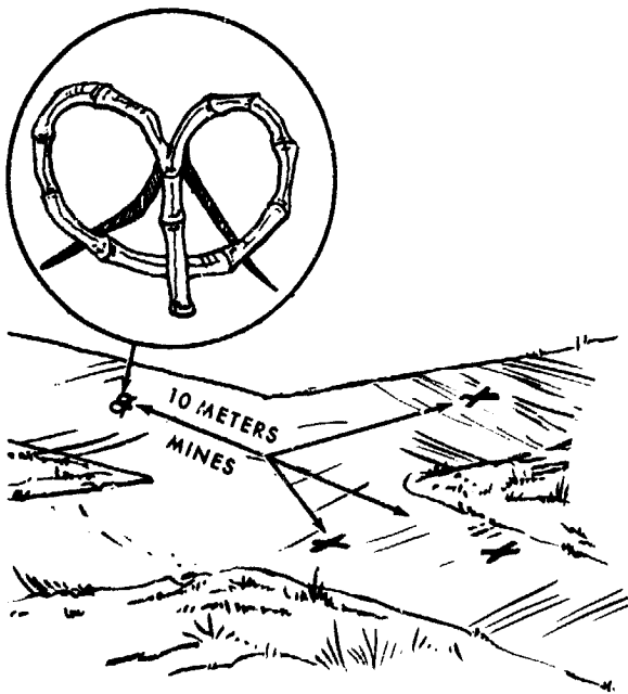
Figure 5-20. Cloverleaf device.
