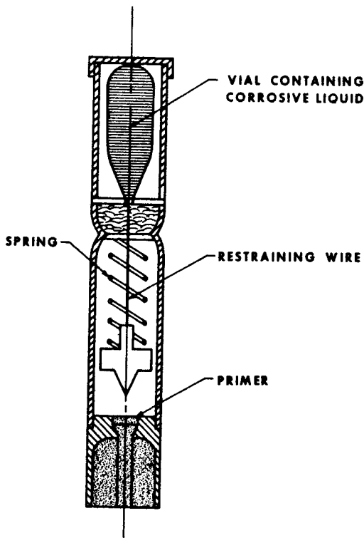
Figure 34. Chemical fuze.
