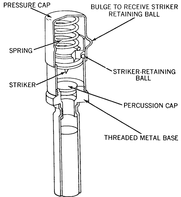
Figure 35. Soviet pressure fuze MV-5.
