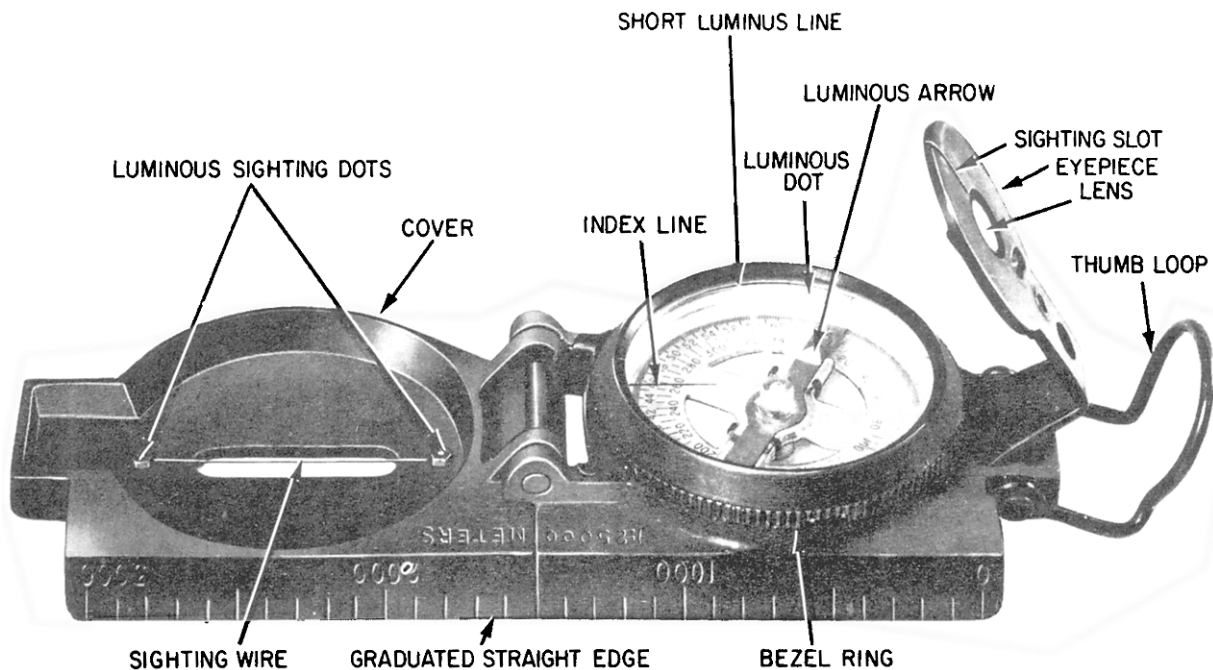
Figure 5-26.—Lensatic compass.
