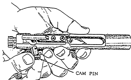
Figure 3-17.—Removing the cam pin.
