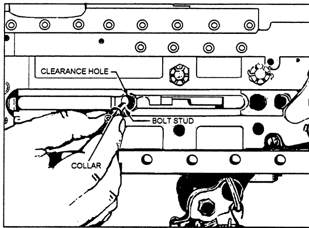
Figure 13-39.—Removing the bolt stud.
