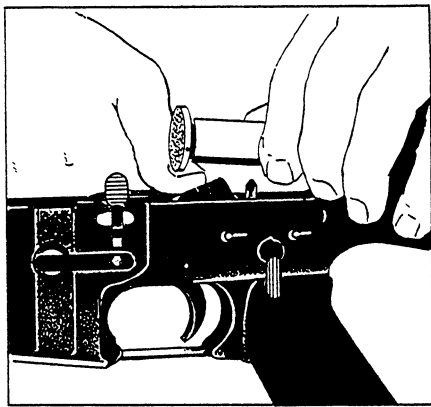
Figure 3-19.—Removing the buffer assembly and action spring.
