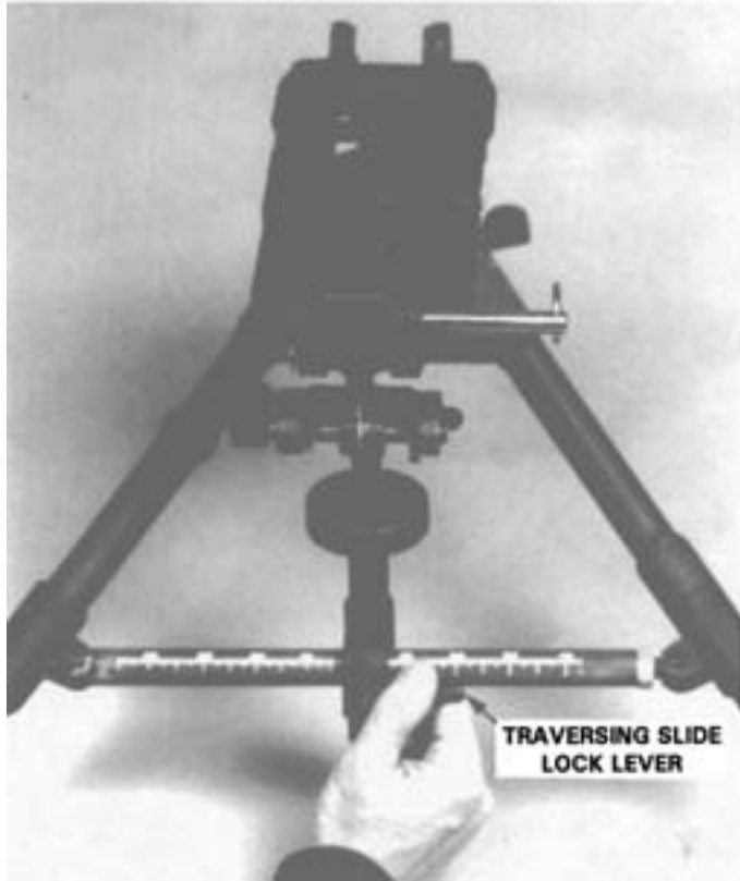
Figure 3-42. Attaching the Flex-mount to the Tripod—Continued.
