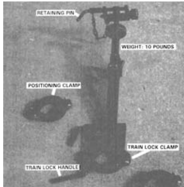
Figure 5-41. T&E Mechanism Mount Assembly.
