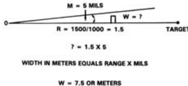
Figure 6-52. Estimating Mask Clearance.
