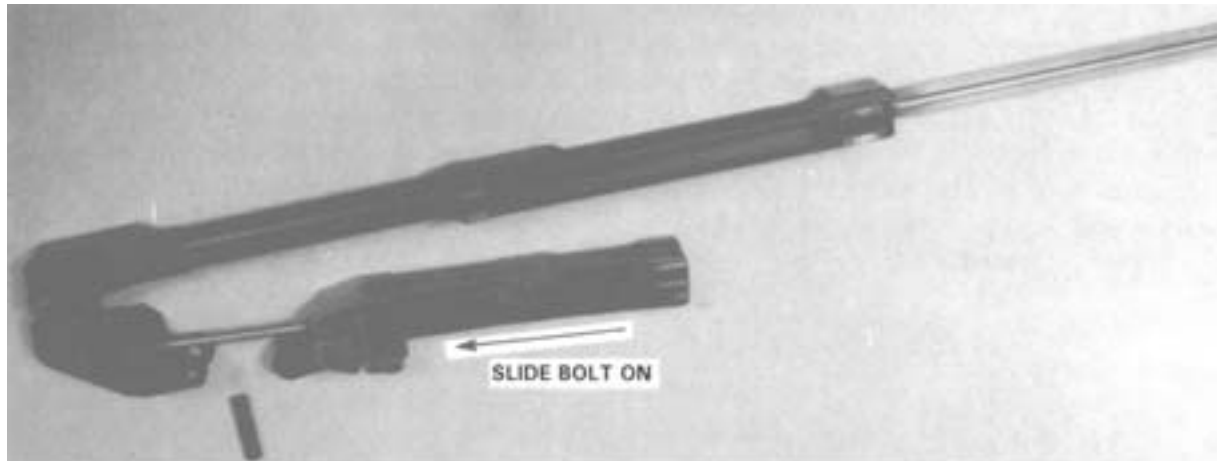
Step 1. Sliding the Bolt Over Firing Pin.
