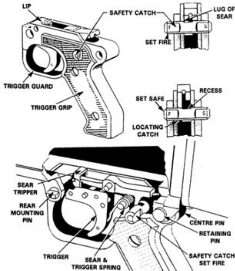
Figure 3-61. Operation of the Safety.
