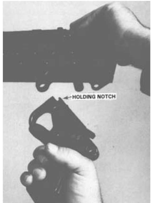
Figure 3-11. Replacing the Trigger Housing Group.
