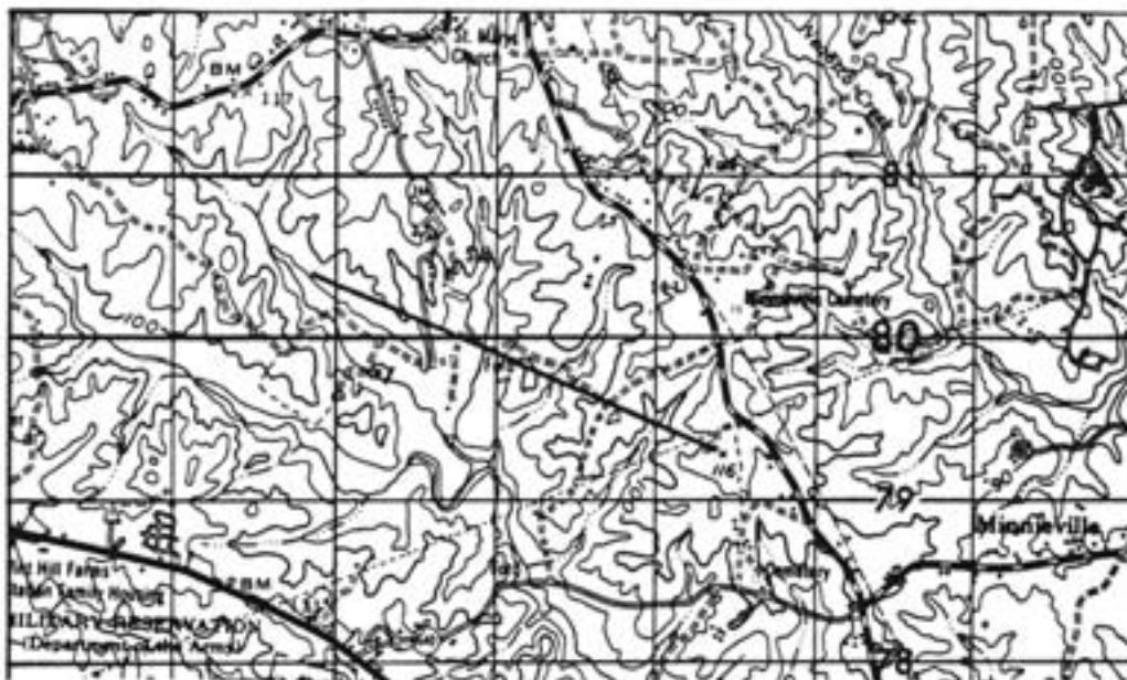
Figure 6-46. Profile Line (Map Contour Interval is 10 Feet).
