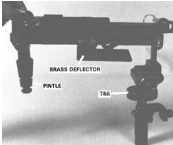
Figure 3-40. Flex-mount.
