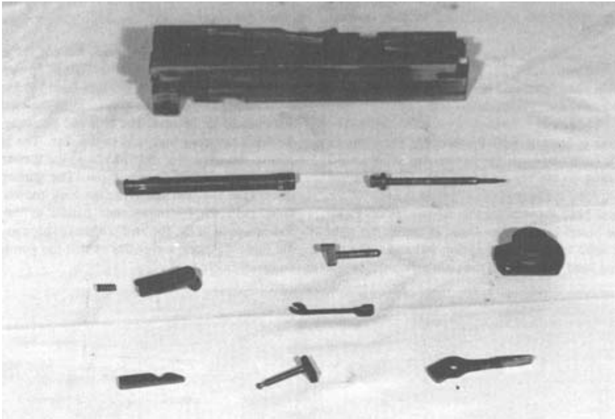
Figure 4-19. Bolt Group, Exploded View.
