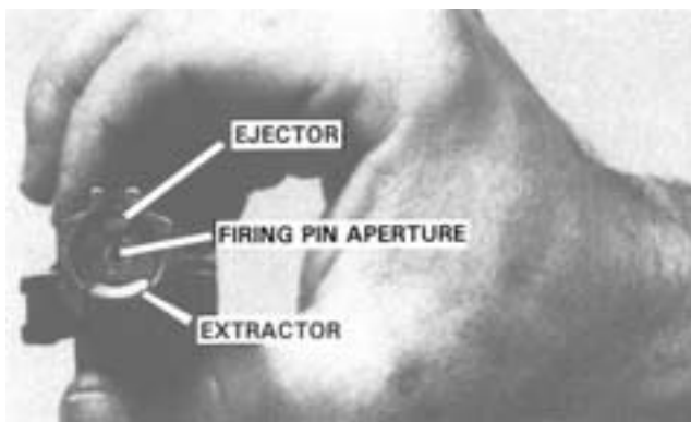
Figure 3-14. Bolt Face.
