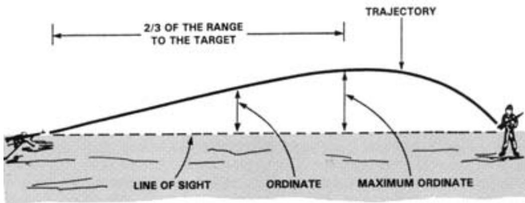
Figure 6-1. Trajectory.
