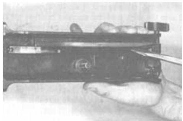
Figure 4-44. Removing the Cover Extractor Spring.
