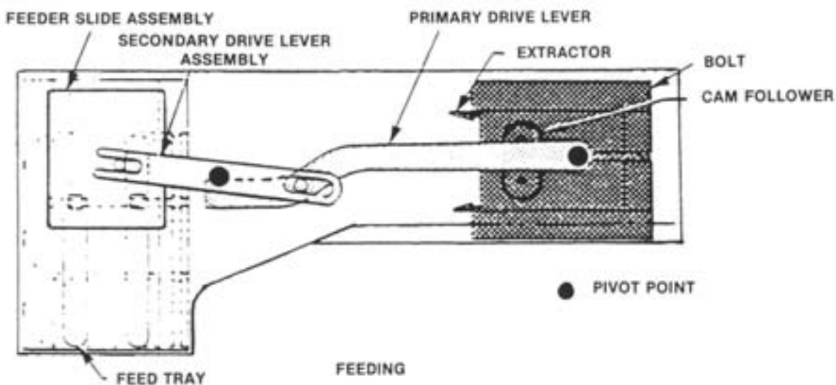
Figure 5-23. Position of Drive Levers, Bolt to Rear.
