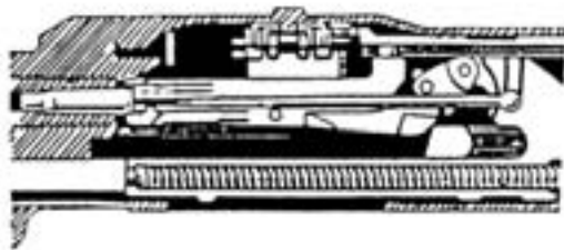
Figure 3-29. Unlocking.
