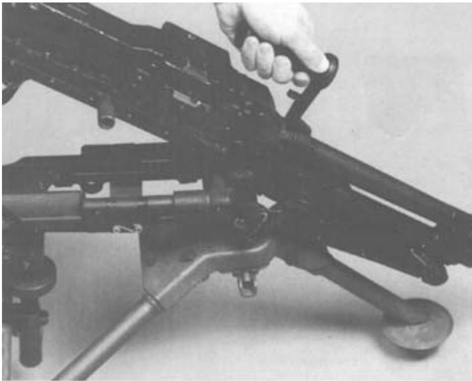
Step 1. Affixing the Gun to the Flex-mount's Forward Bushing.
