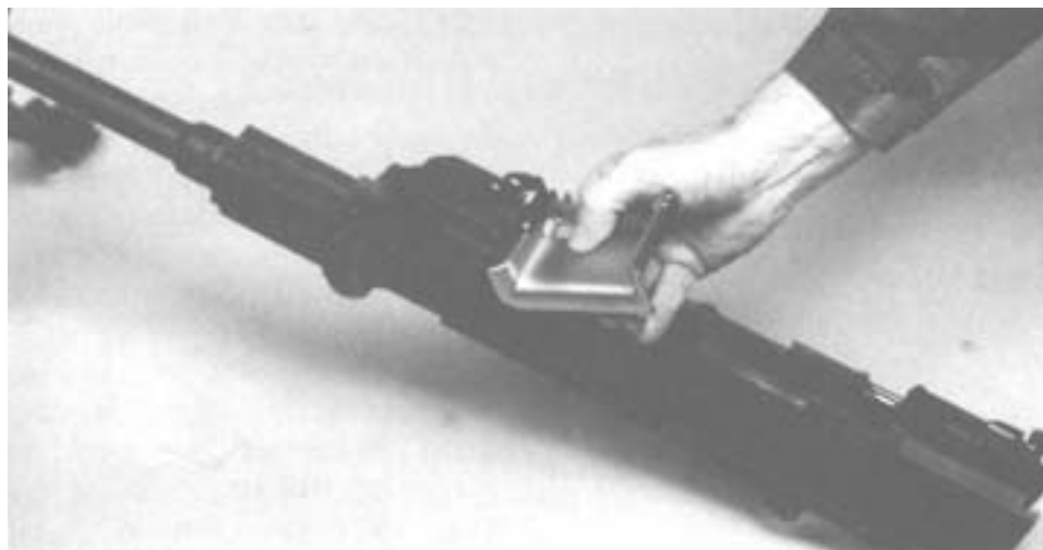
Figure 3-21. Aligning the Feed Tray Guides.
