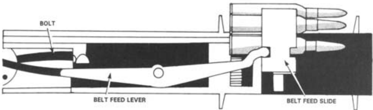
Figure 4-58. Belt Feed Slide Moving Out of the Side of the Cover.
