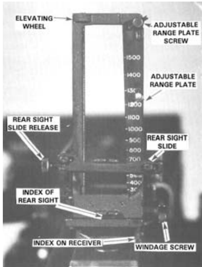
Figure 5-3. Rear Sight.
