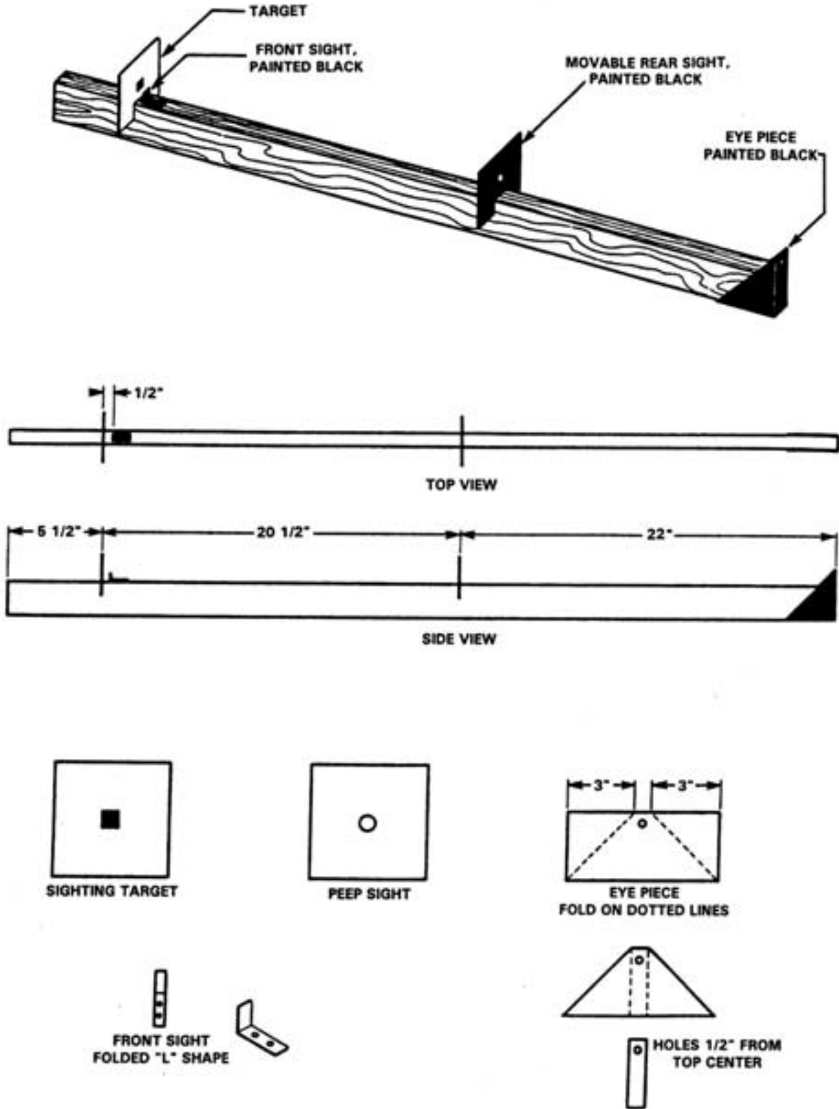
Figure 4-107. Sighting Bar.
