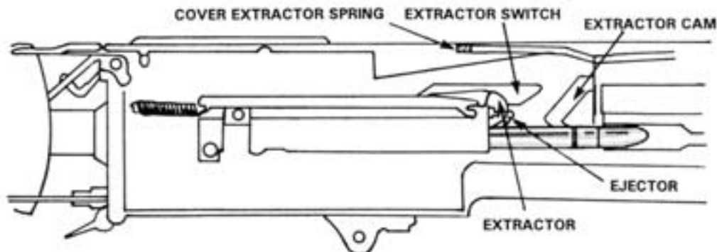
Figure 4-62. Chambering.
