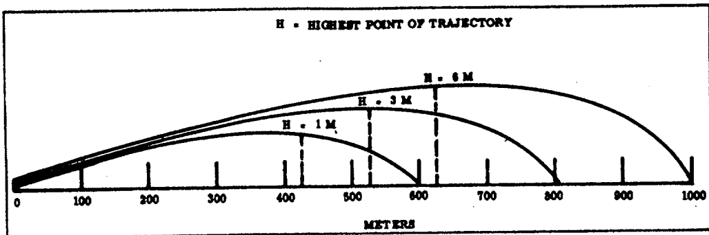
Figure 2-3. Diagram Showing Maximum Ordinate (H) of Trajectory.
