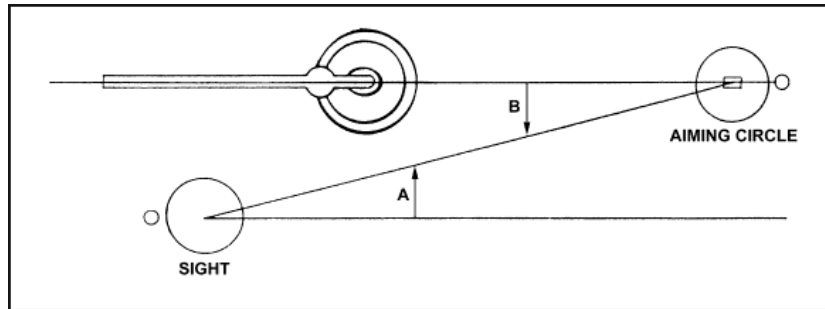
Figure 2-19. Calibration for deflection using the angle method.
