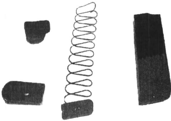
Figure 1-26. Disassembled Magazine.
