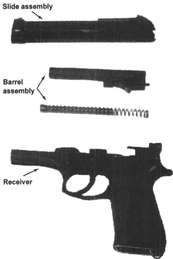
Figure 1-4. Major Components.
